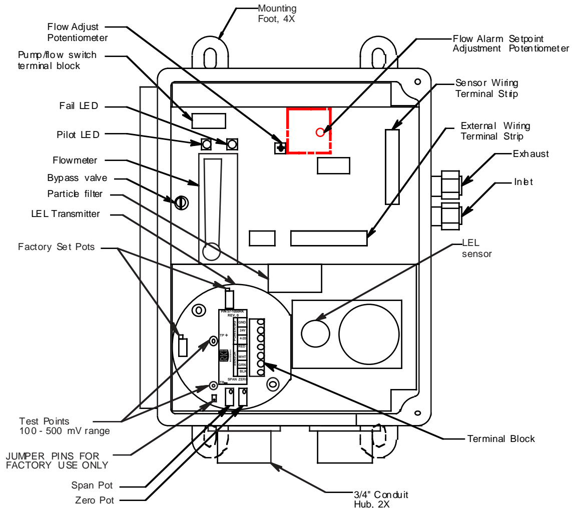
Figure 1: Sample draw Combustible Gas Detector Component Location
