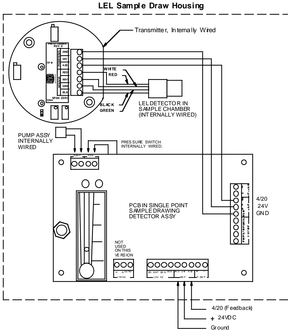
Figure 4: Wiring the Sample Draw Combustible Gas Detector
