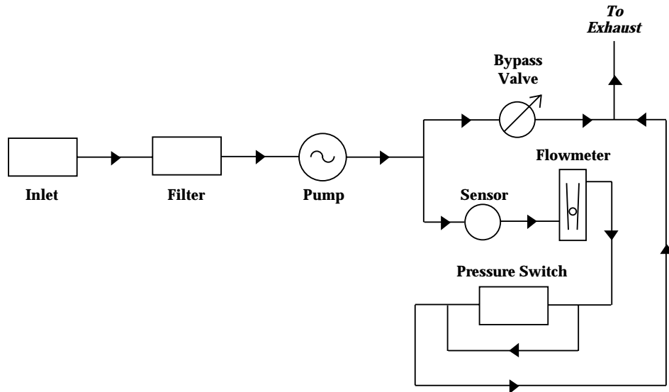
Figure 2: Sample draw Combustible Gas Detector Flow Diagram
