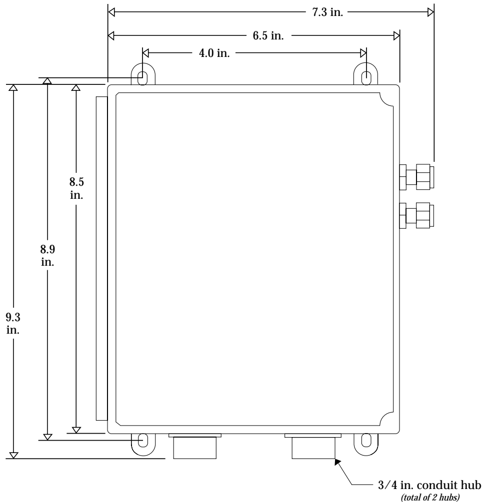
Figure 3: Mounting the Sample Draw Combustible Gas Detector
