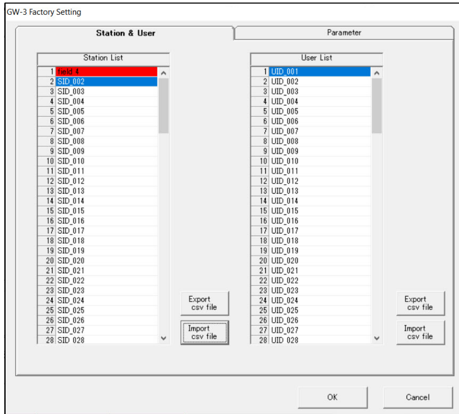
Figure 16: Station & User Tab with Invalid Custom ID
