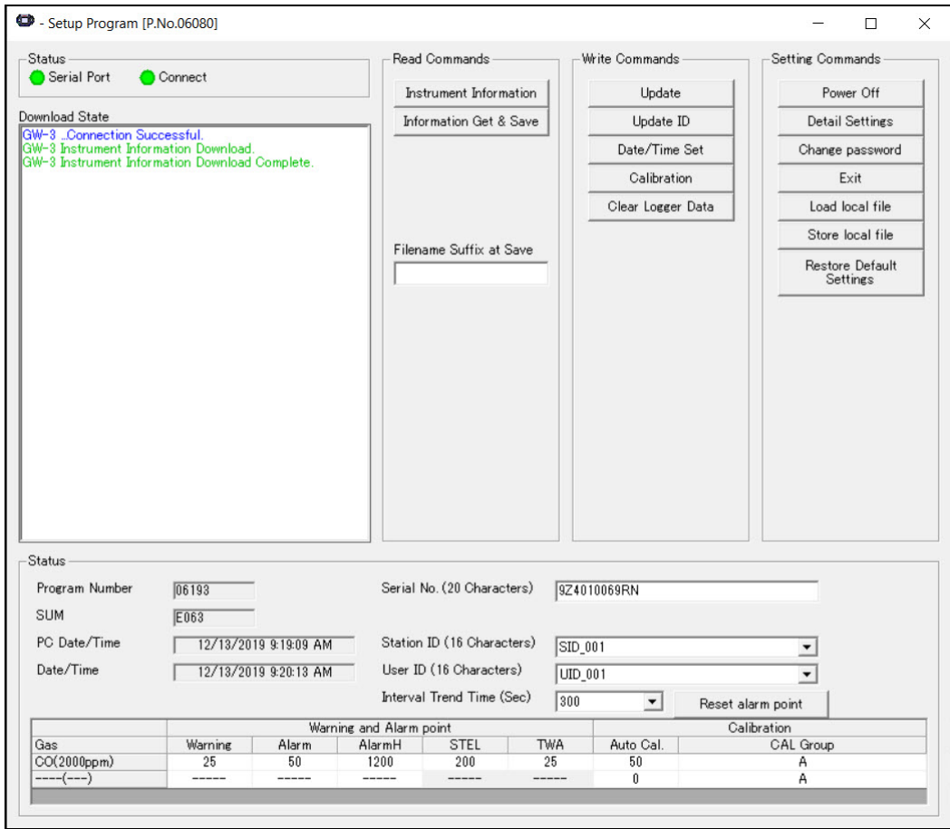
Figure 7: Main Window
