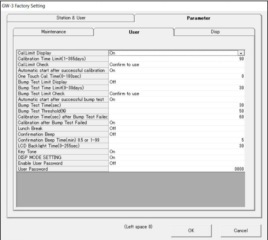
Figure 9: Parameter\User Tab
