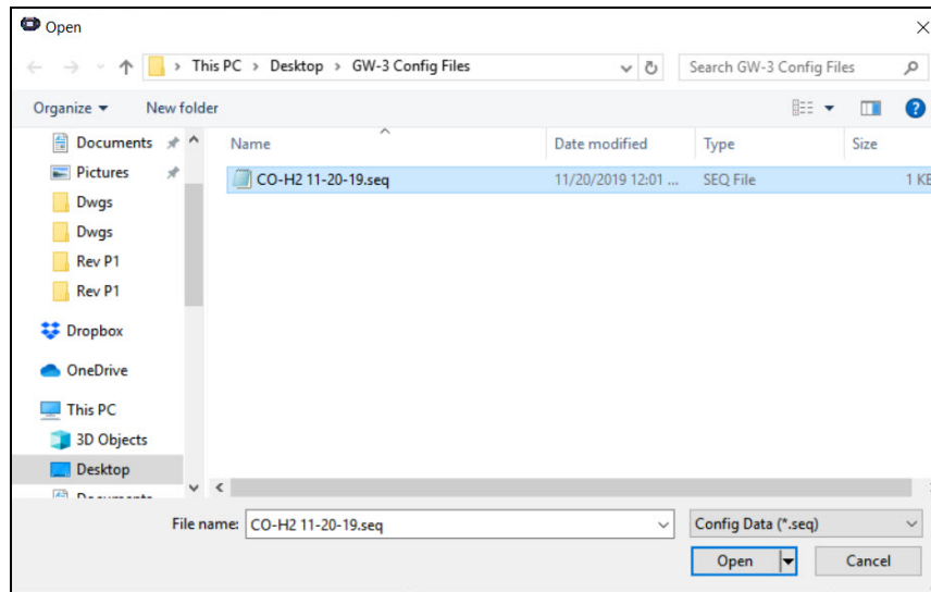
Figure 19: Open Window
