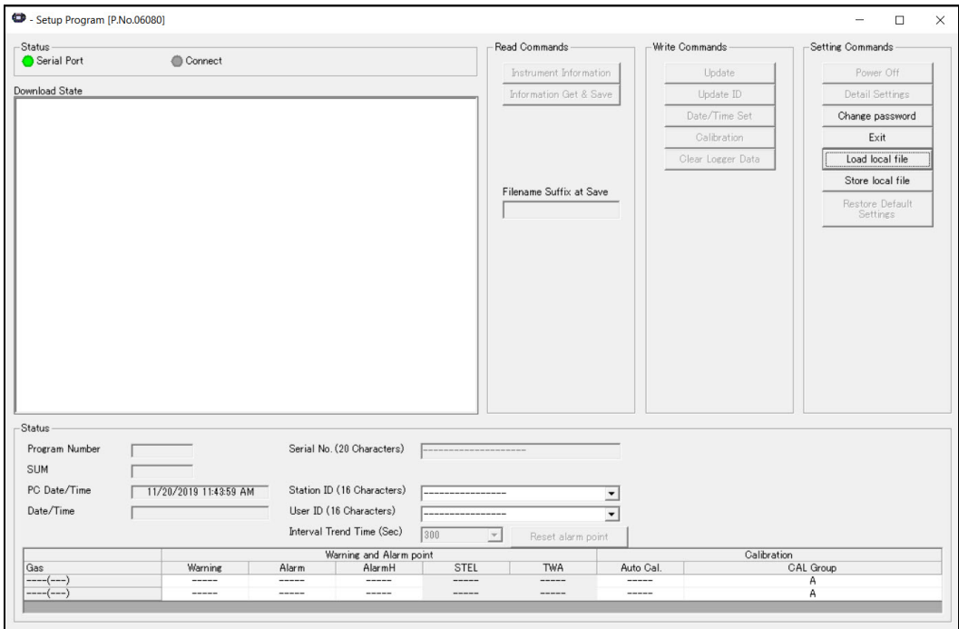
Figure 3: Main Window
