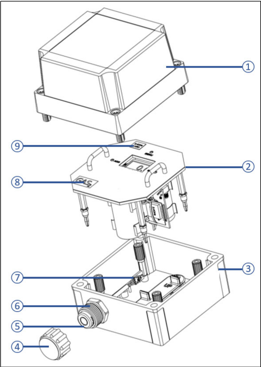
Figure 3: Exploded Diagram
