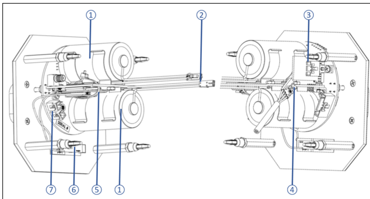
Figure 2: Internal Component Location
