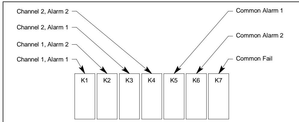
Figure 5. Beacon 200 Channel Relay Allocation
