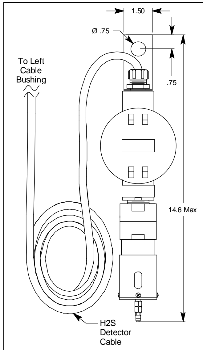
Figure 7. H 2 S Detector Outline and Mounting Dimensions
