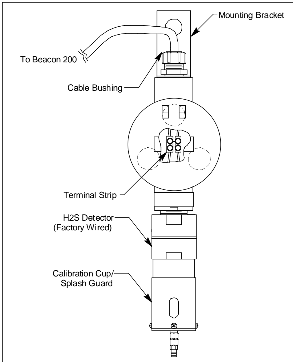
Figure 2. H 2 S Junction Box Component Location
