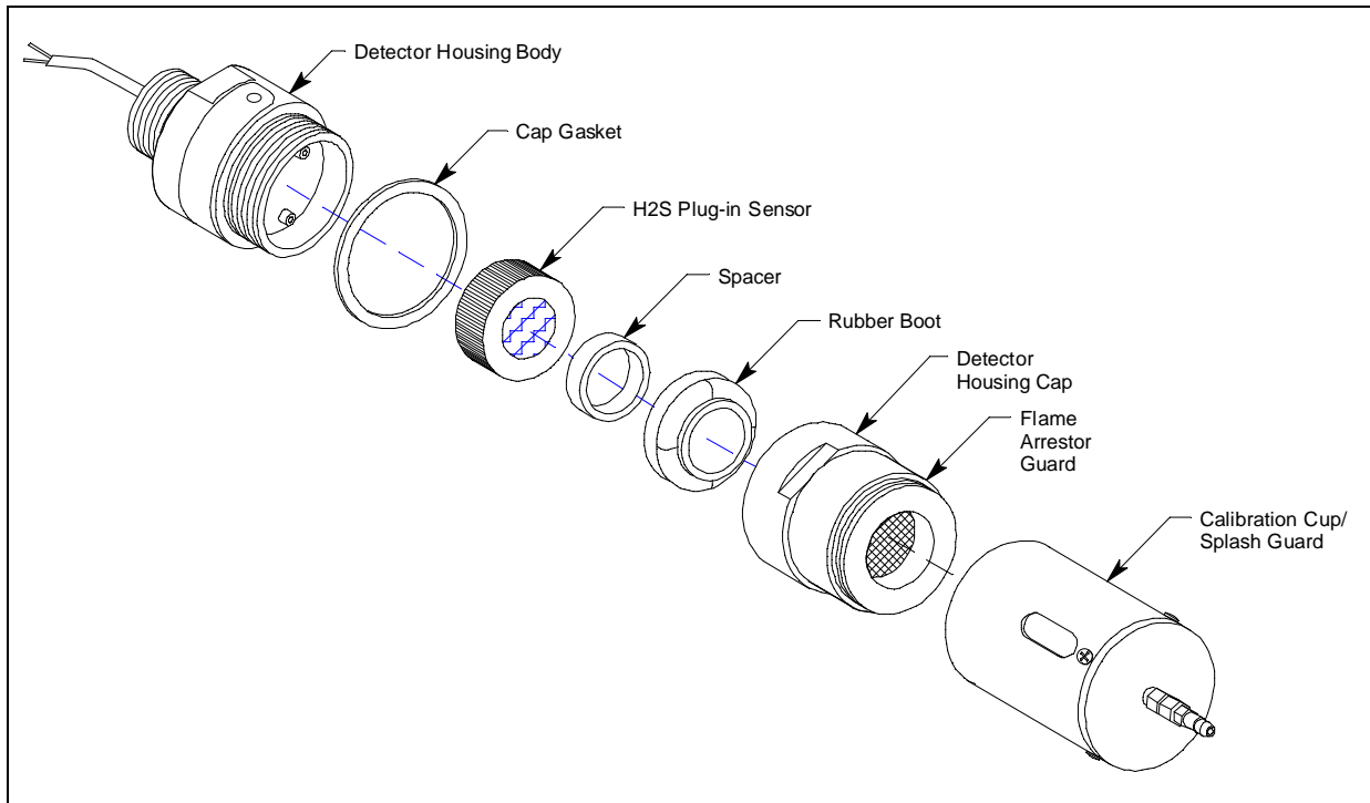
Figure 3. H 2 S Detector Component Location
