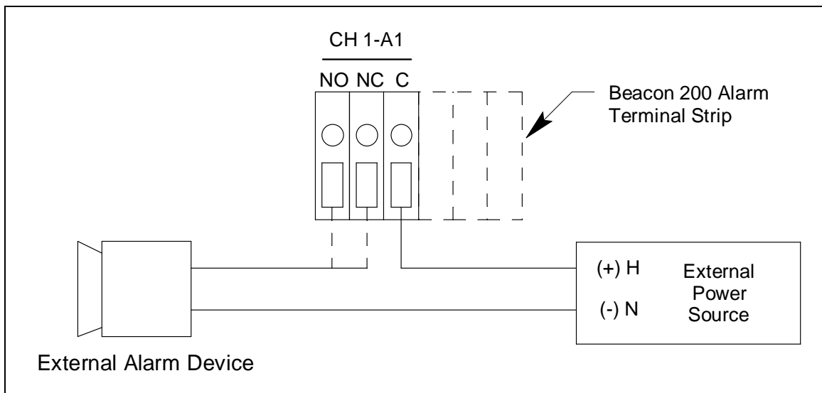
Figure 10. Typical External Alarm Wiring, Single Device
