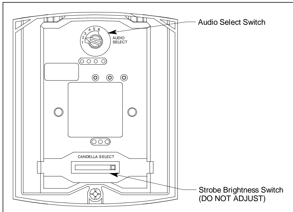
Figure 15. Strobe/Horn Cover
