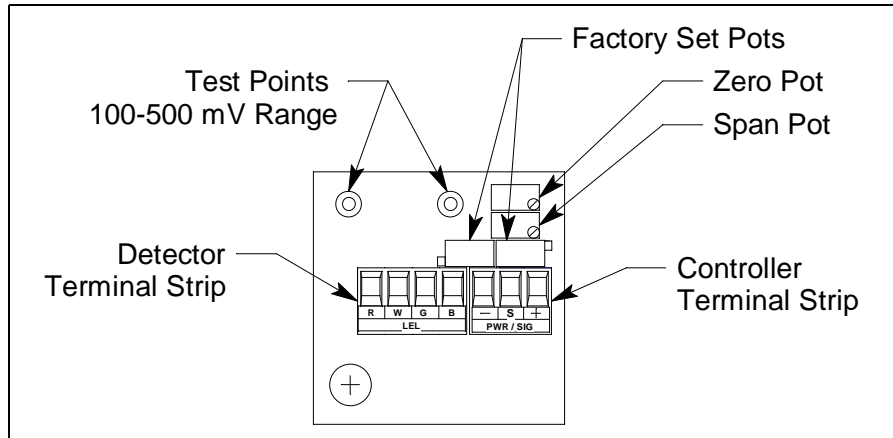
Figure 3: Amplifier Component Location
