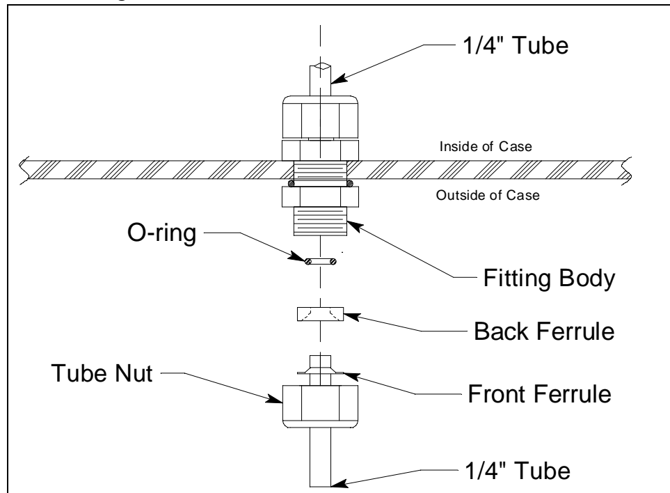
Figure 6: Inlet Fitting with Tubing Stub
