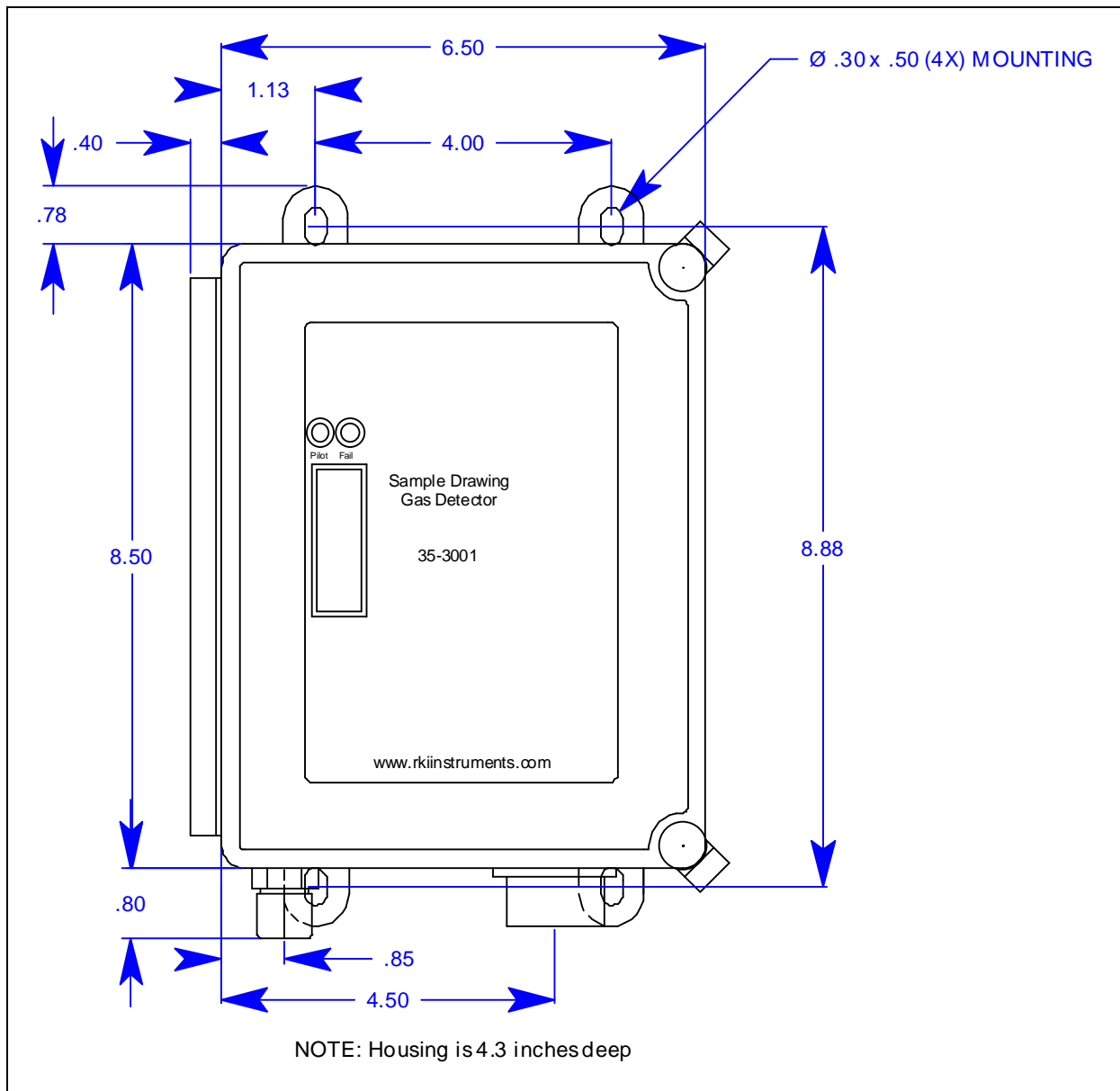
Figure 4: Outline and Mounting Dimensions
