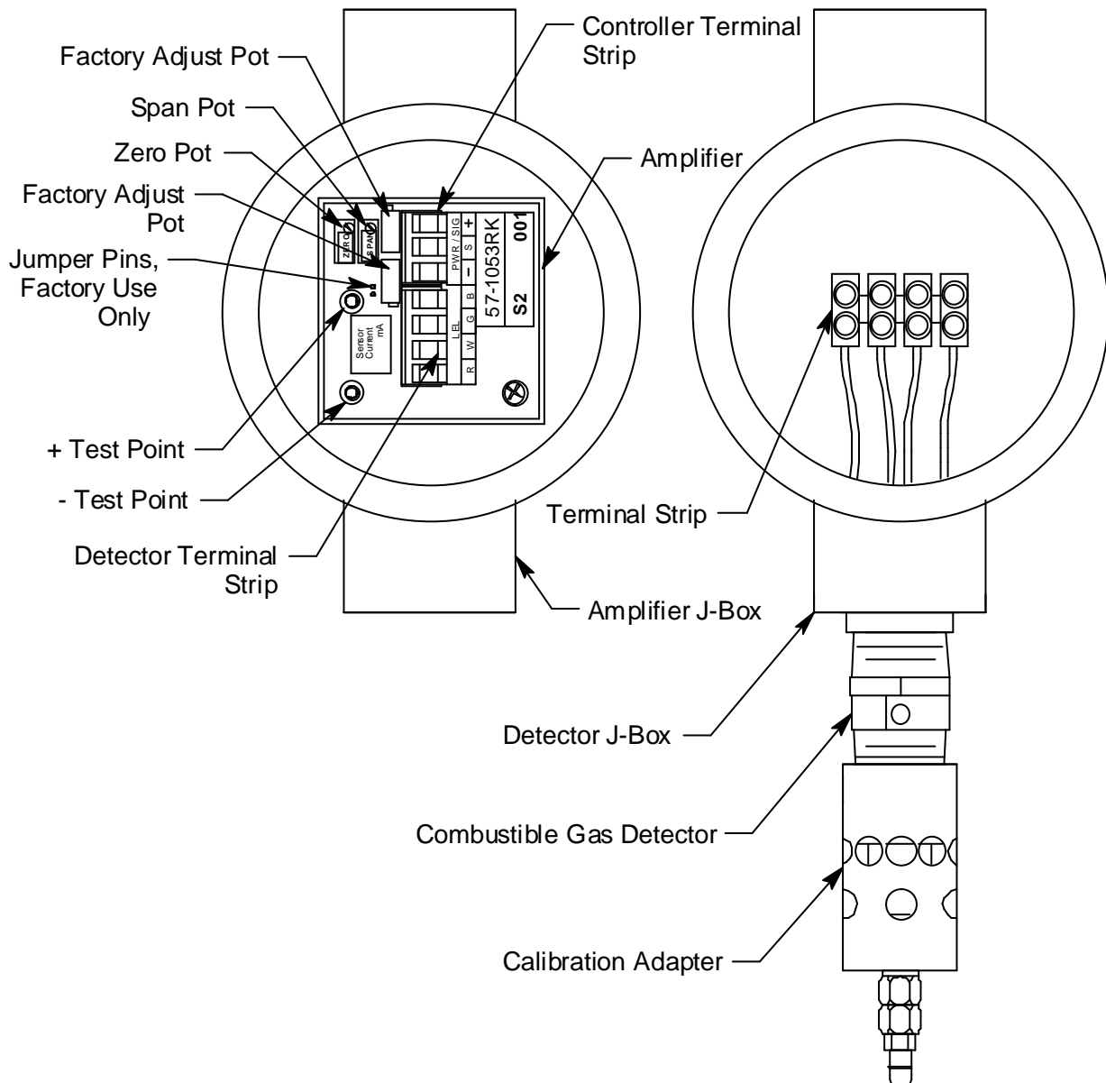
Figure 1: Combustible Gas Transmitter Component Location
