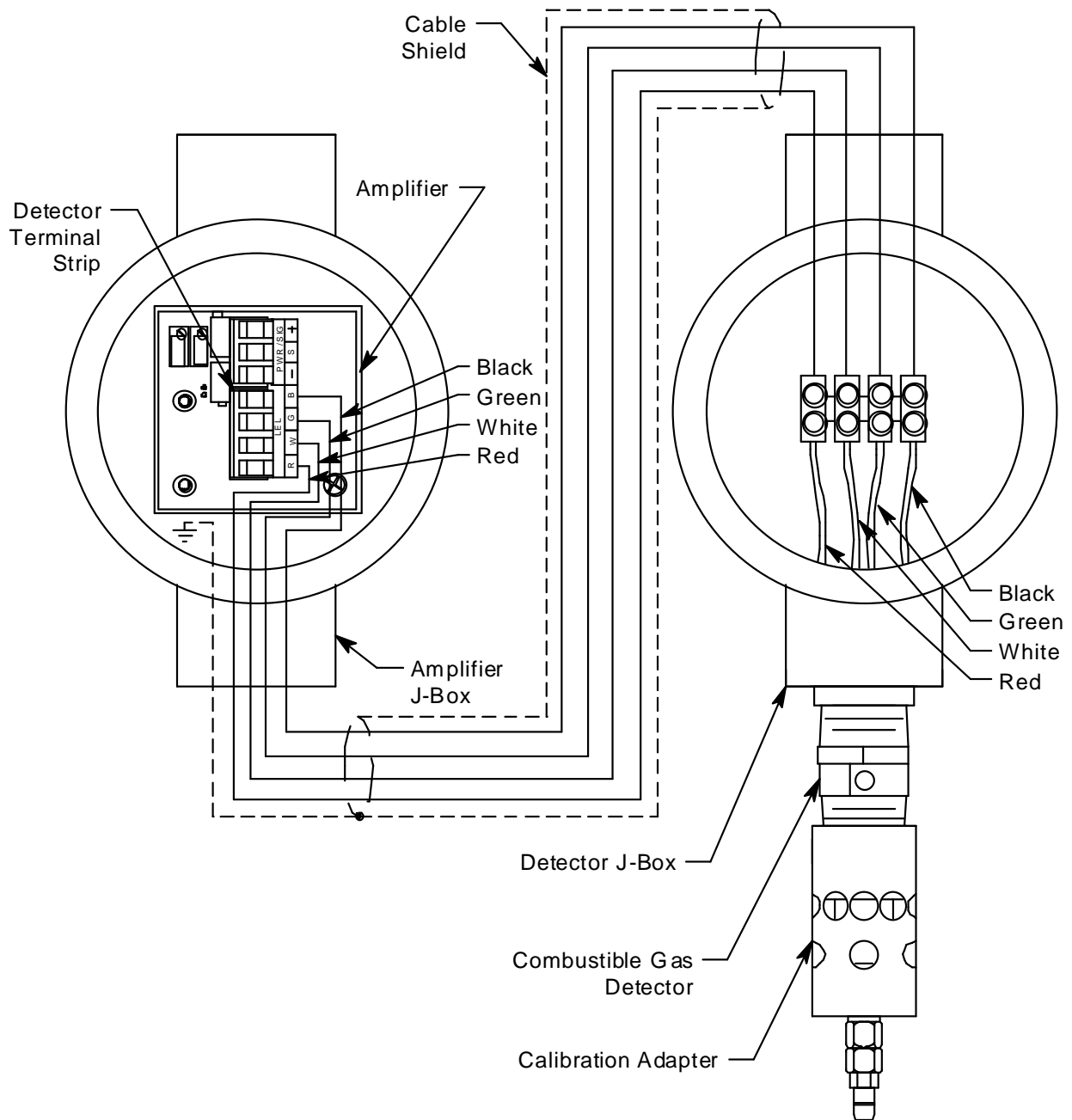
Figure 3: Wiring the Detector to the Amplifier
