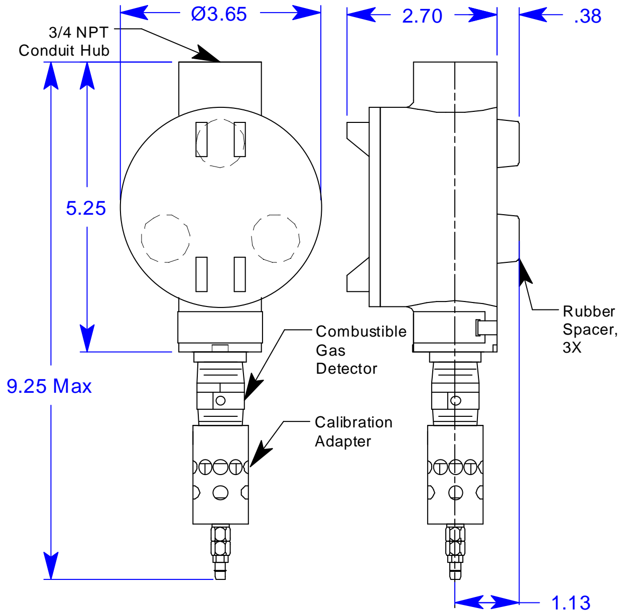
Figure 2: Mounting the Combustible Gas Transmitter
