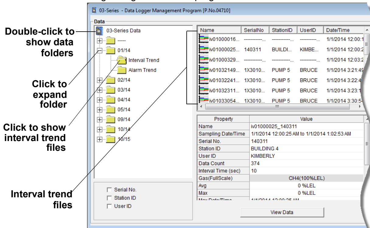
Figure 18: Data Window, Basic Data Organization
