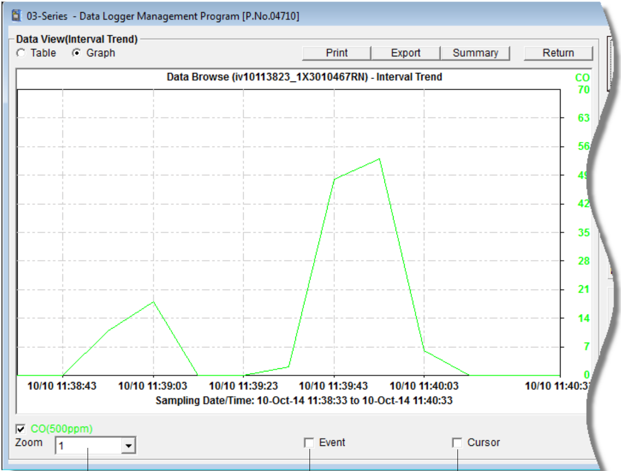
Figure 36: Interval Trend Data in Graph Format
