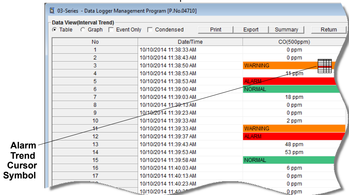
Figure 34: Alarm Trend Cursor Symbol
