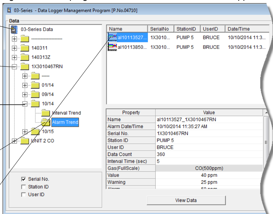
Figure 39: Data Window - Selecting Alarm Trend Data Files
