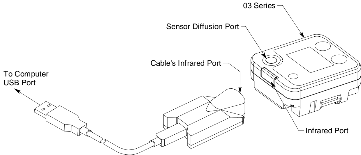
Figure 13: Aligning the 03 Series with the Cable Infrared Receiver
