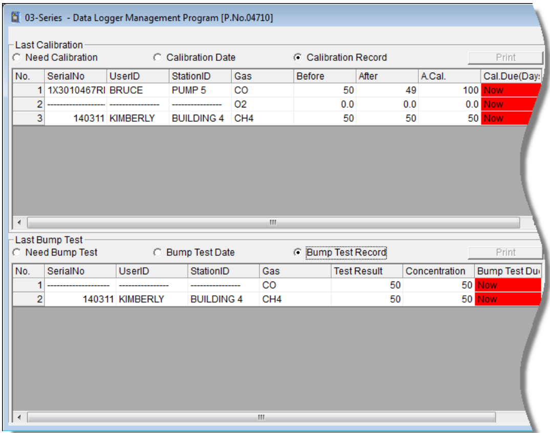
Figure 59: Last Calibration Window: Calibration Record View Option
