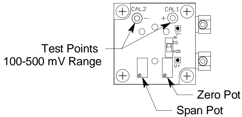
Figure 3: CO Amplifier Component Location
