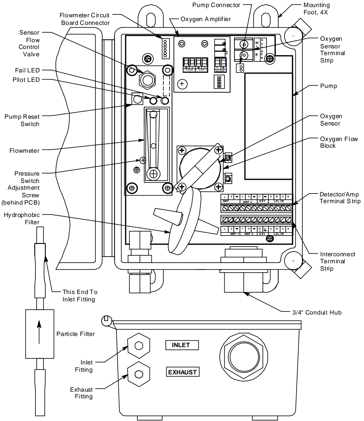
Figure 1: Oxygen Sample-Draw Detector Component Location
