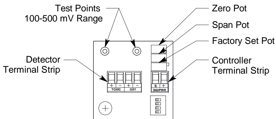
Figure 3: Amplifier Component Location
