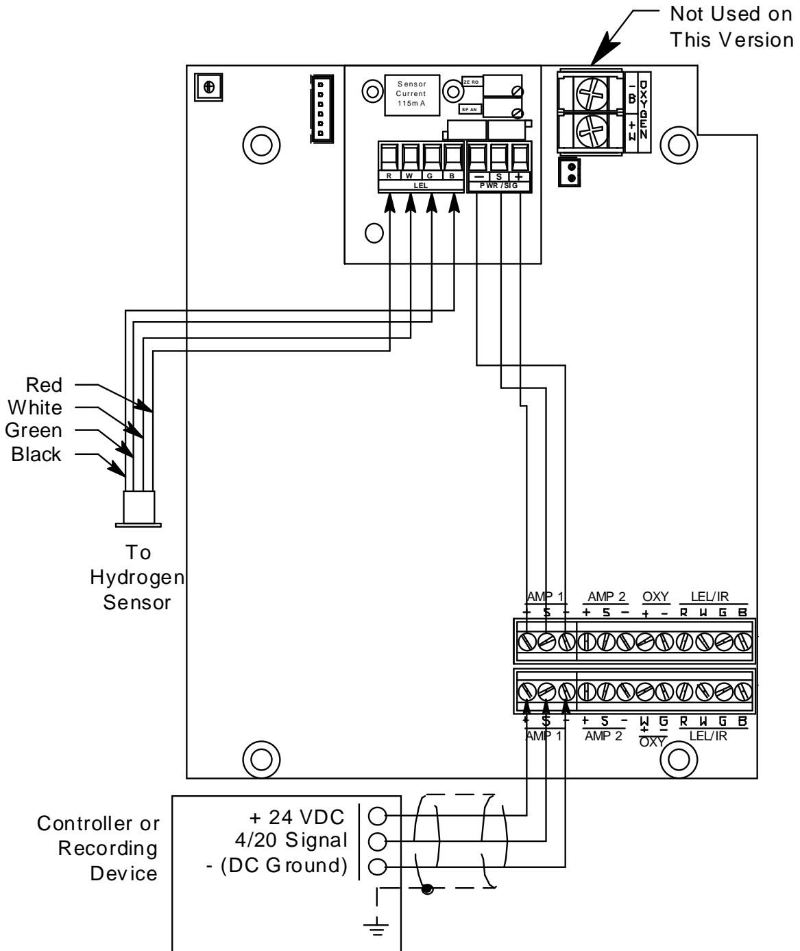
Figure 5: Wiring the Sample-Draw Detector to a Controller
