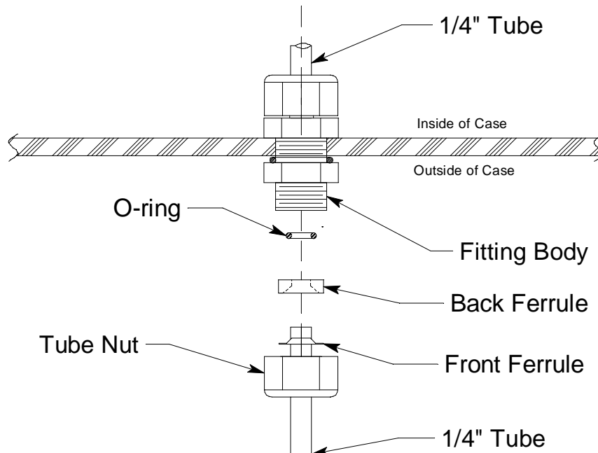
Figure 6: Inlet Fitting with Tubing Stub
