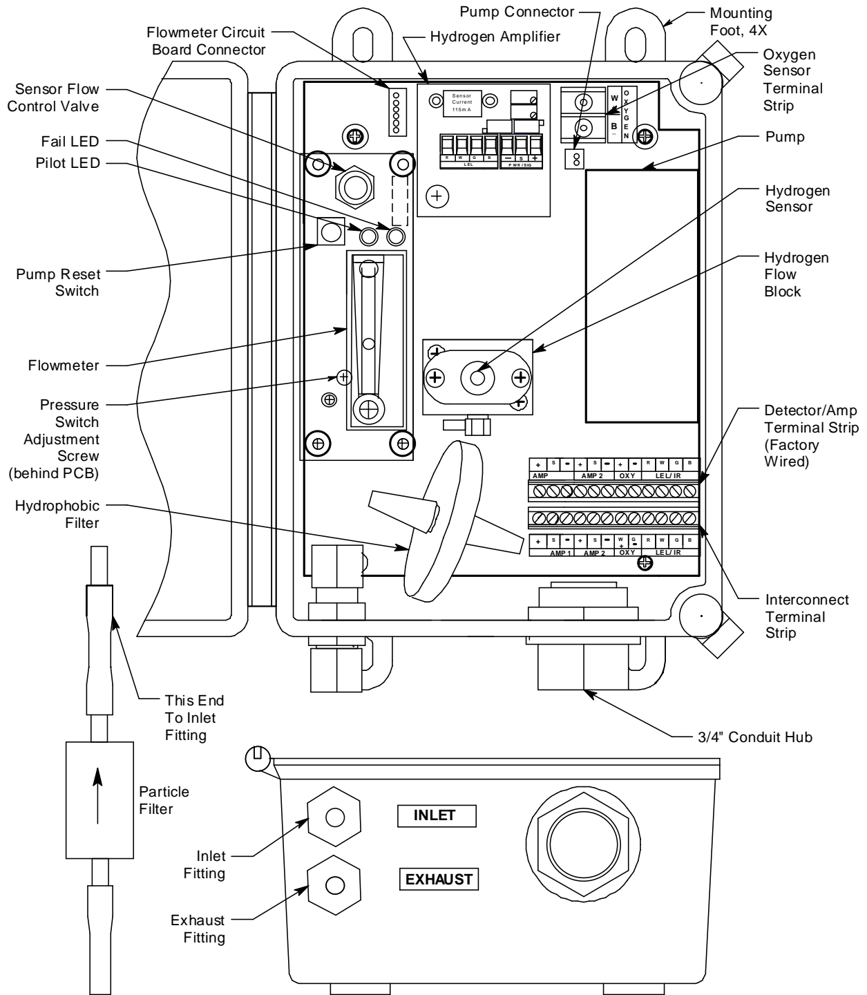
Figure 1: Hydrogen Sample-Draw Detector Component Location
