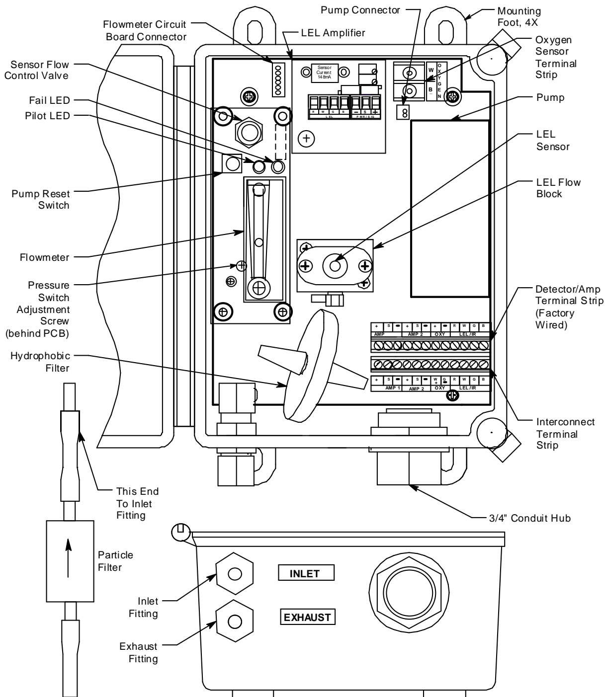
Figure 1: Combustible Gas Sample-Draw Detector Component Location
