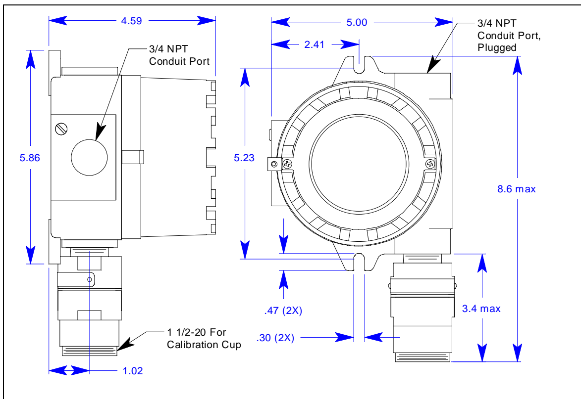
Figure 19: Outline & Mounting Dimensions, H 2 S, CO, HCN, and Oxygen, CSA, Explosion-Proof
