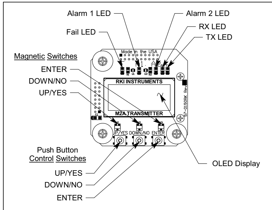
Figure 13: Control PCB Component Location
