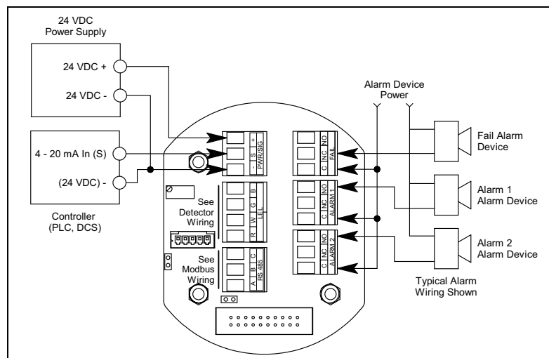
Figure 37: PLC and DCS Device Wiring
