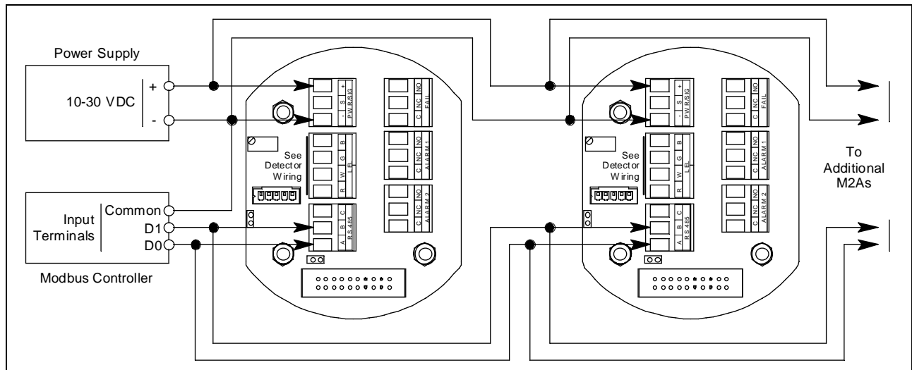
Figure 34: Alternate Modbus Wiring
