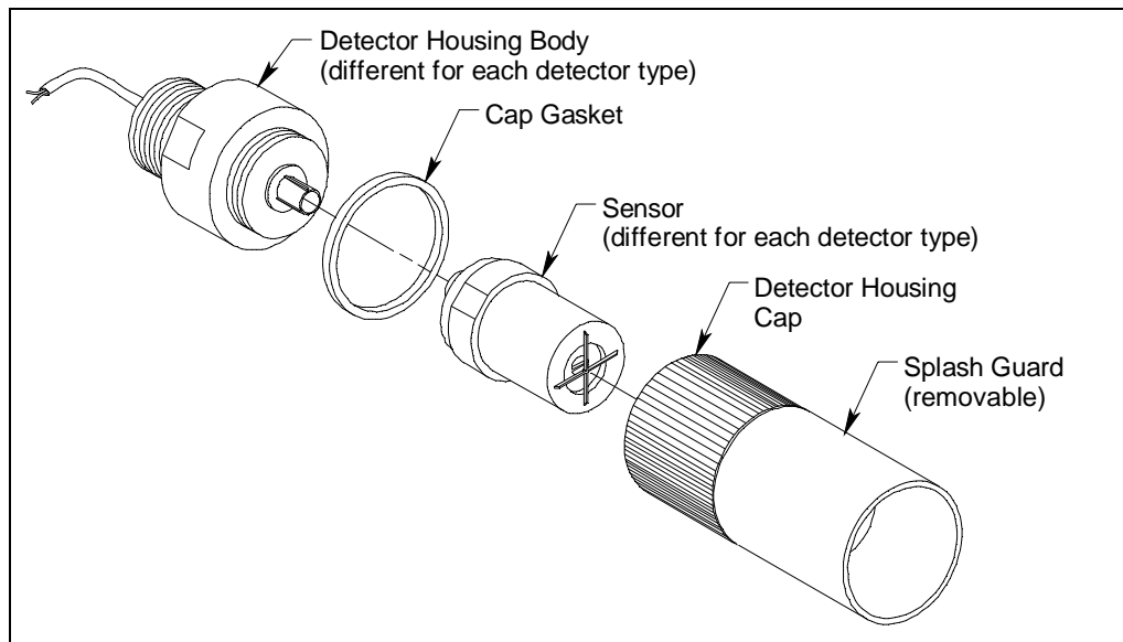
Figure 2: Toxic Detector Component Location
