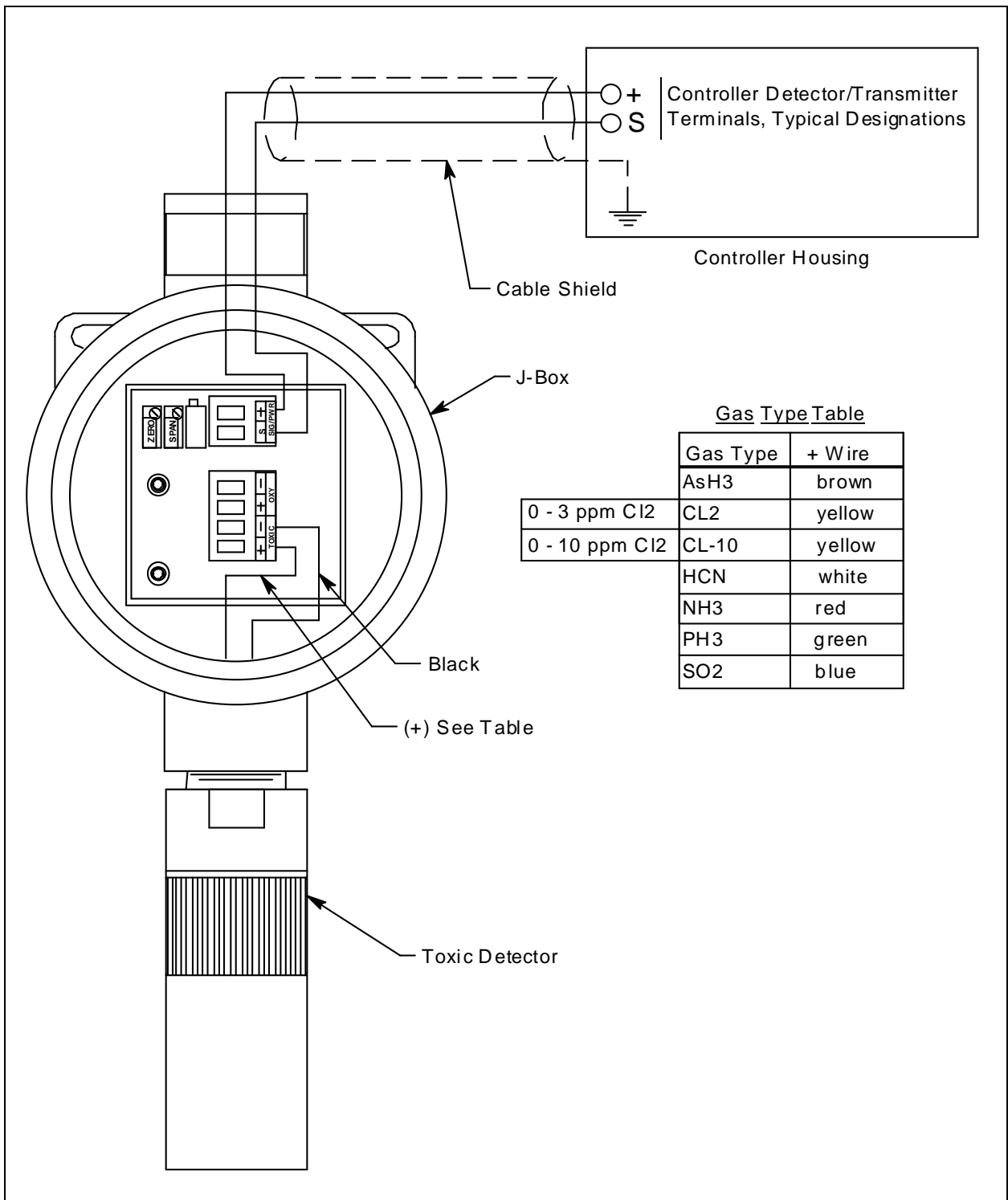
Figure 5: Wiring the Toxic Gas Transmitter to a Controller
