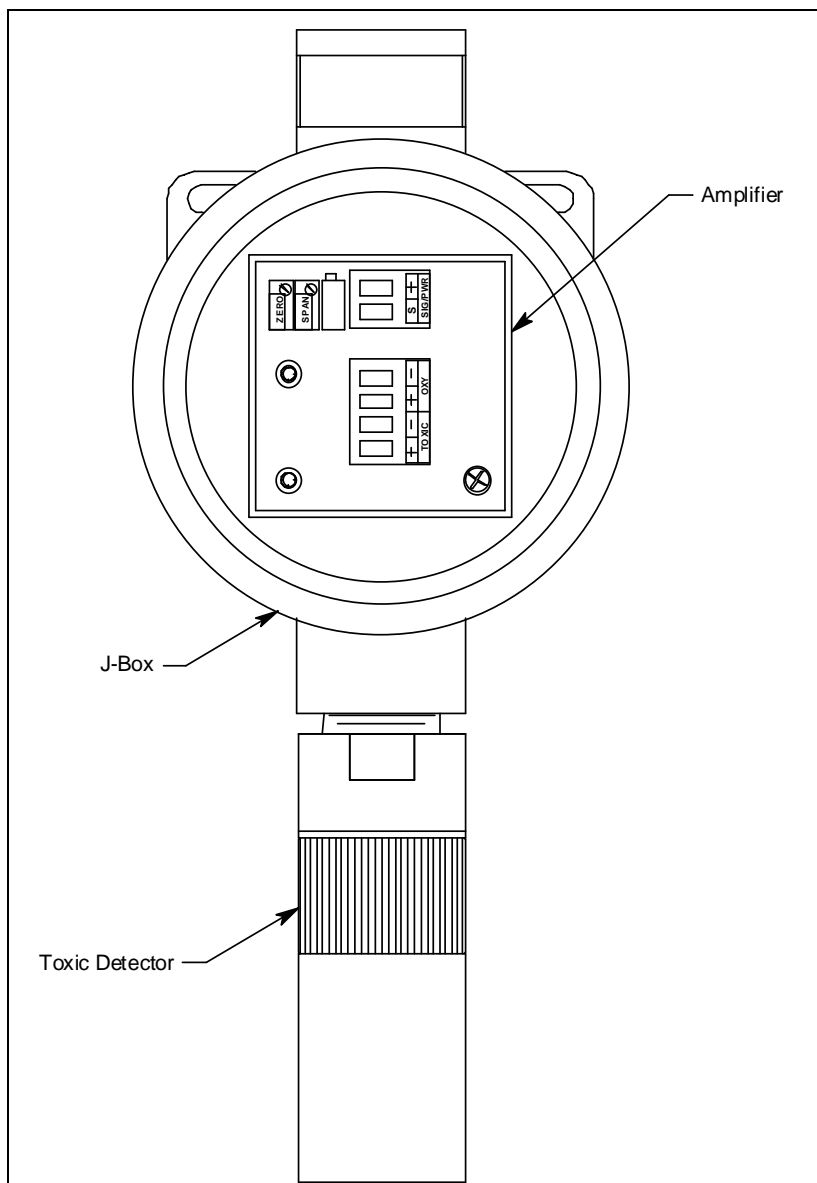
Figure 1: Toxic Transmitter Component Location
