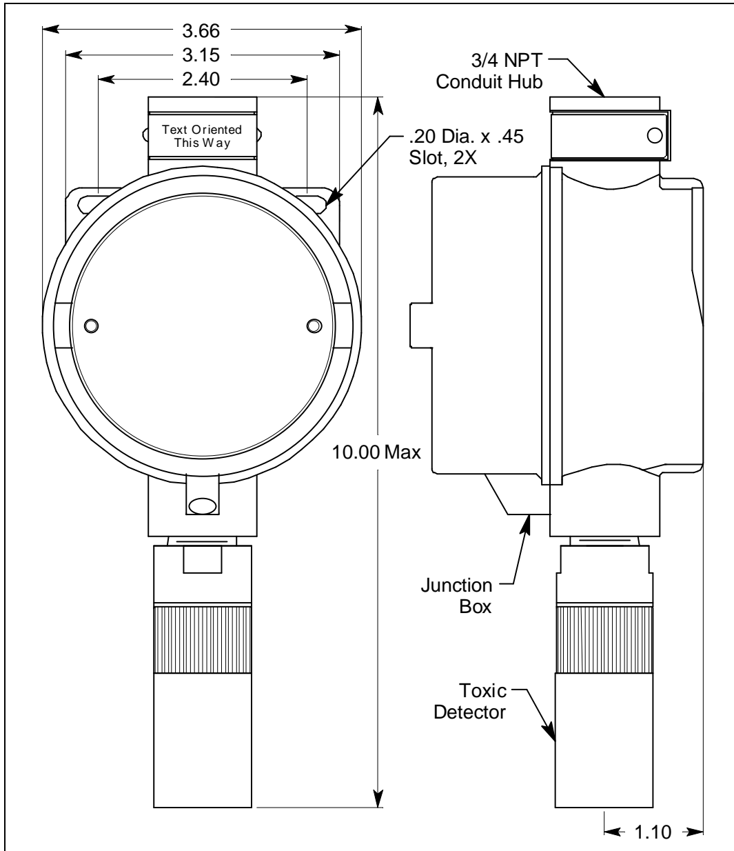
Figure 4: Mounting the Toxic Gas Transmitter
