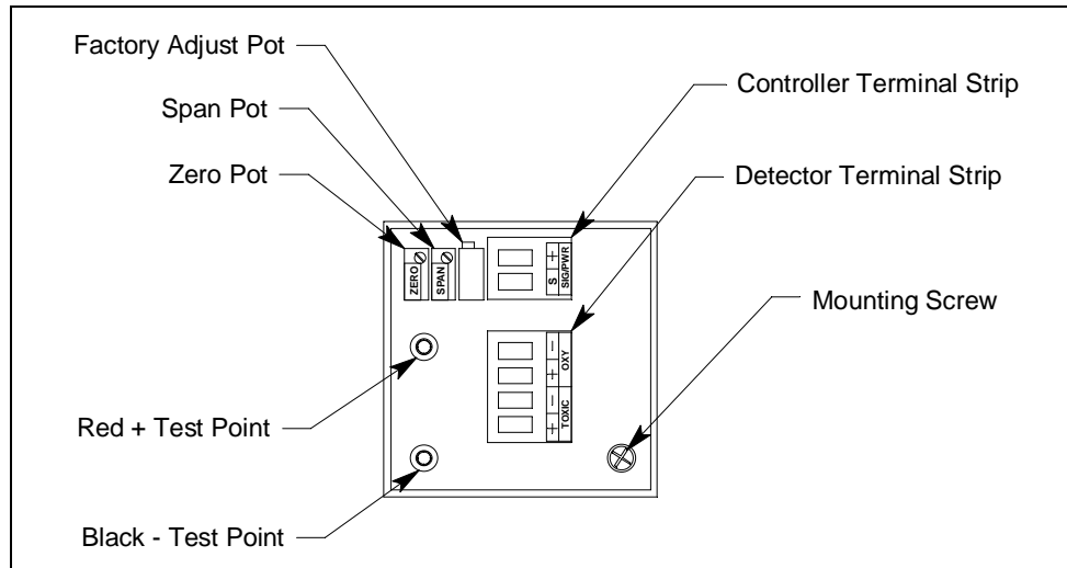
Figure 3: Amplifier Component Location
