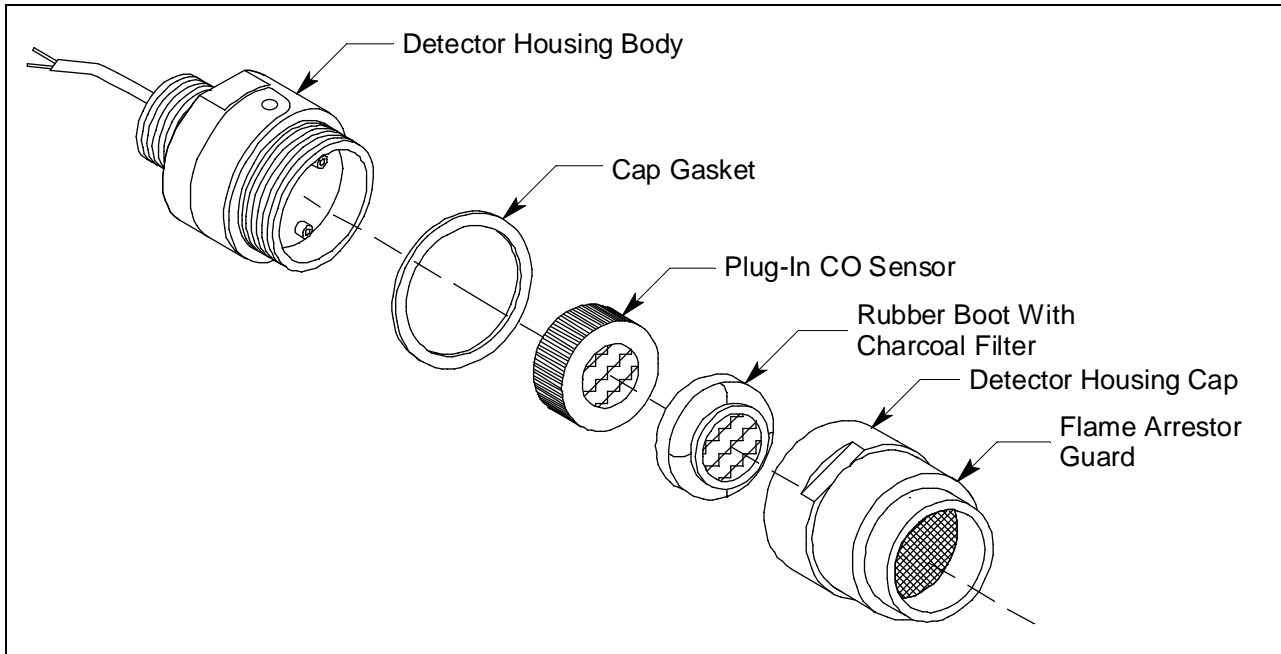
Figure 5: CO Detector Component Location
