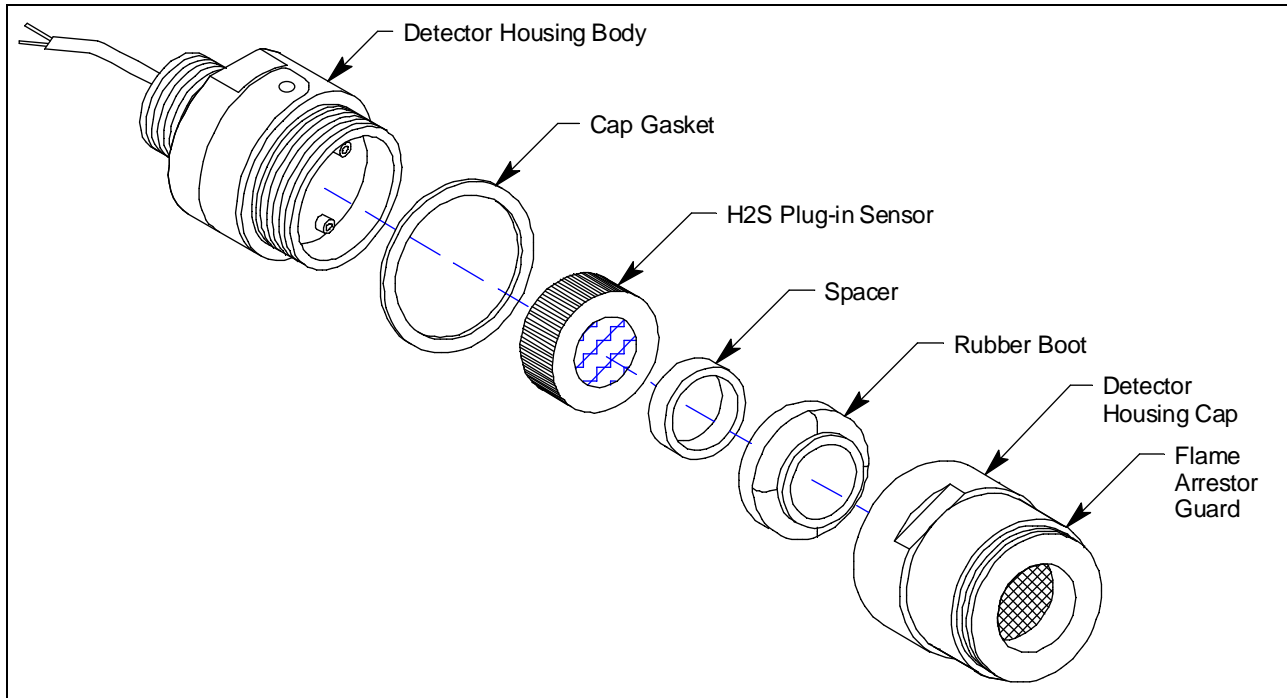
Figure 4: H 2 S Detector Component Location
