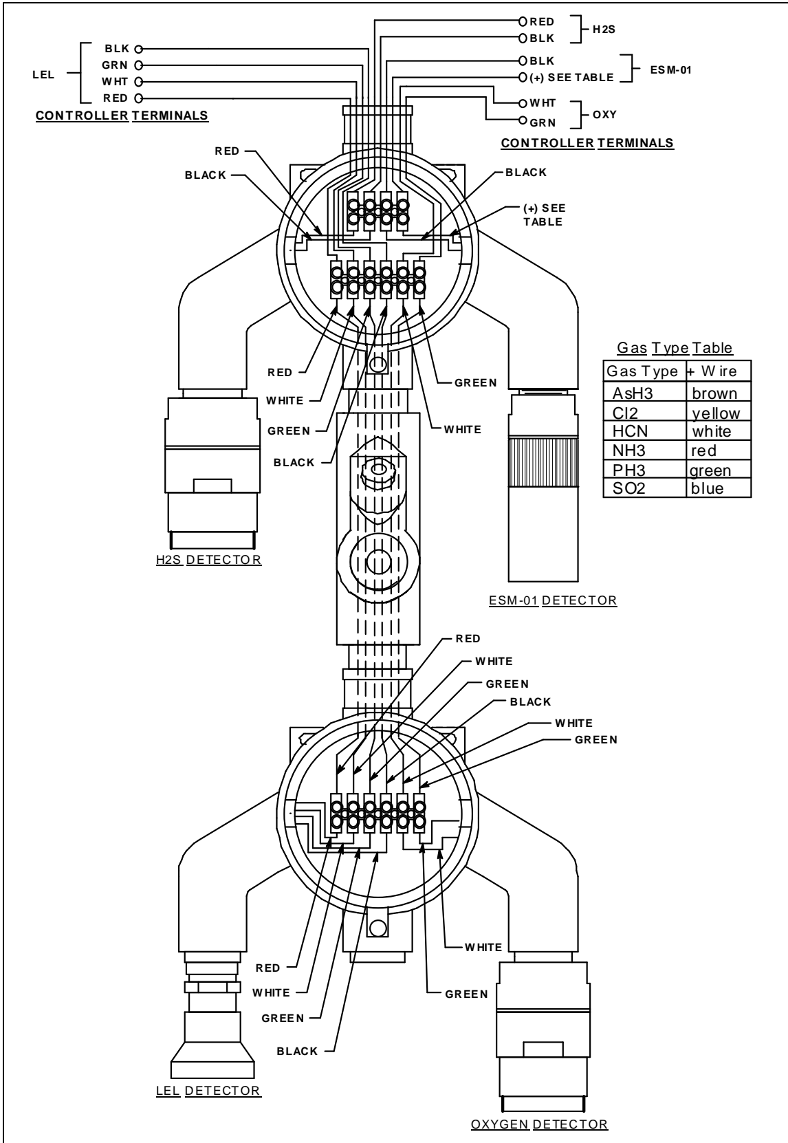
Figure 9: Wiring for Catalytic LEL/O 2 /H 2 S/ESM-01 Versions (65-2484RK-0X)
