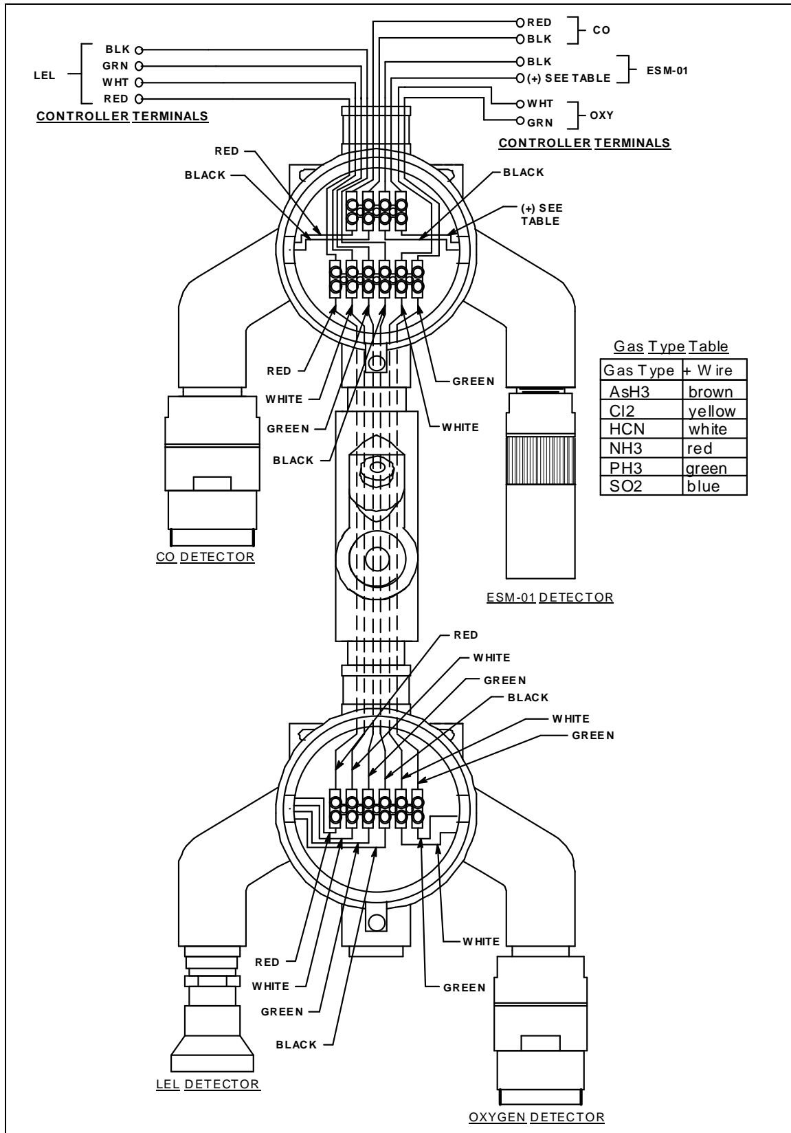
Figure 13: Wiring for Catalytic LEL/O 2 /CO/ESM-01 Versions (65-2484RK-4X)
