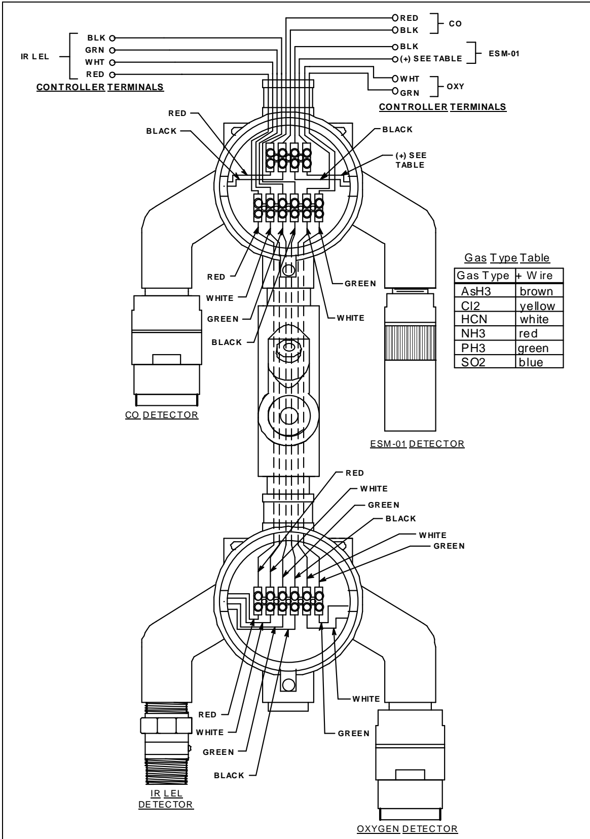
Figure 14: Wiring for IR LEL/O 2 /CO/ESM-01 Versions (65-2484RK-5X)
