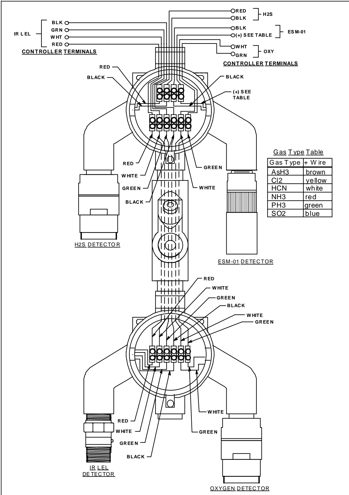
Figure 10: Wiring for IR LEL/O 2 /H 2 S/ESM-01 Versions (65-2484RK-1X)
