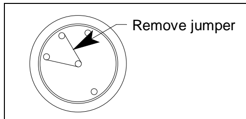
Figure 15: Plug-In Sensor Jumper Removal
