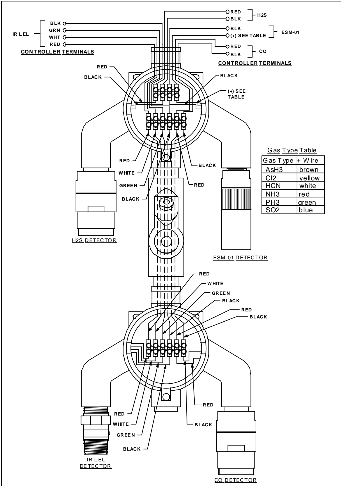
Figure 12: Wiring for IR LEL/CO/H 2 S/ESM-01 Versions (65-2484RK-3X)
