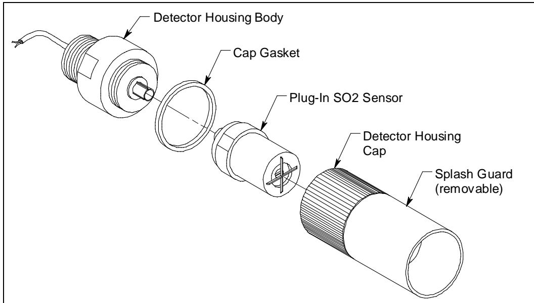
Figure 6: ESM-01 Toxic Detector Component Location
