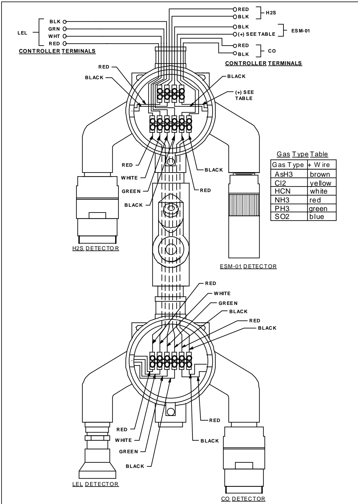
Figure 11: Wiring for LEL/CO/H 2 S/ESM-01 Versions (65-2484RK-2X)
