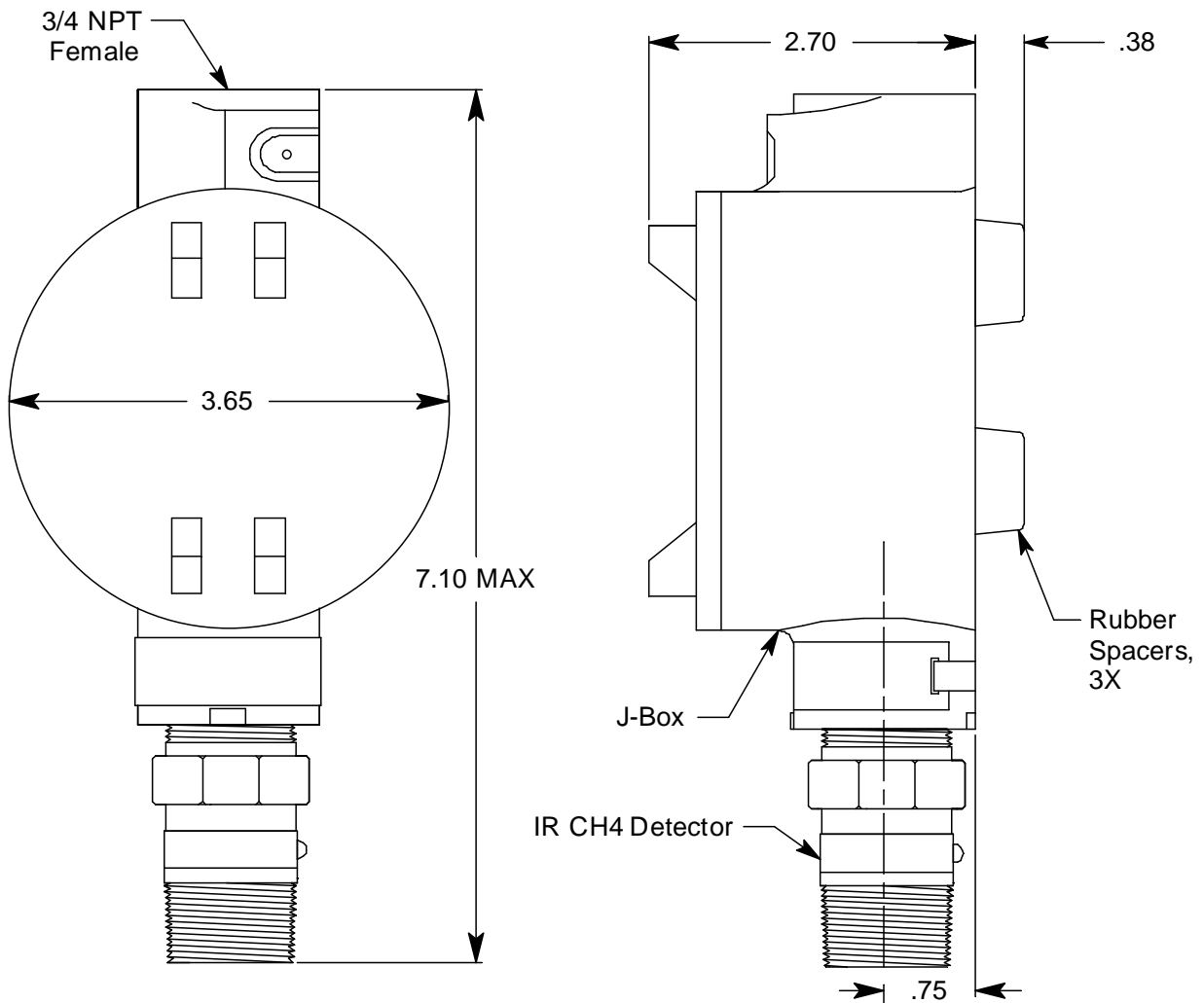
Figure 2: Mounting the Methane Detector
