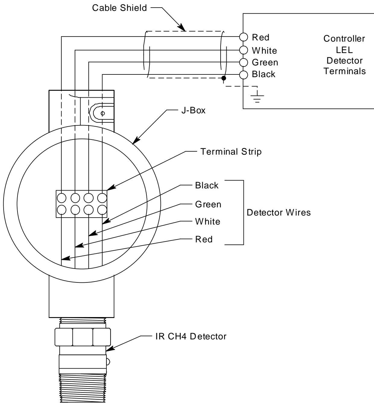
Figure 3: Wiring the Methane Detector to a Controller
