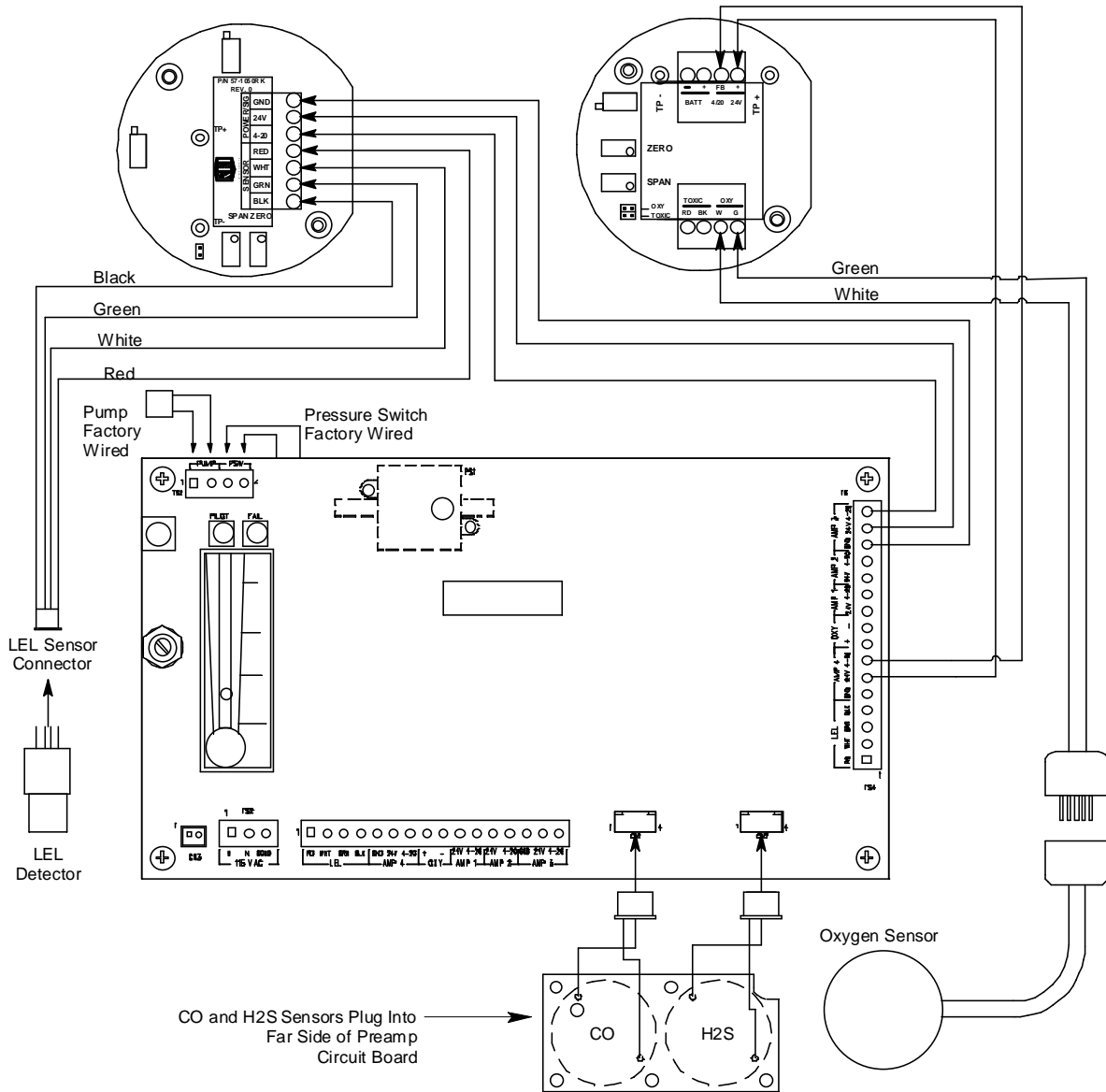
Figure 9: Internal (Factory) Wiring, Sample-Draw Detector
