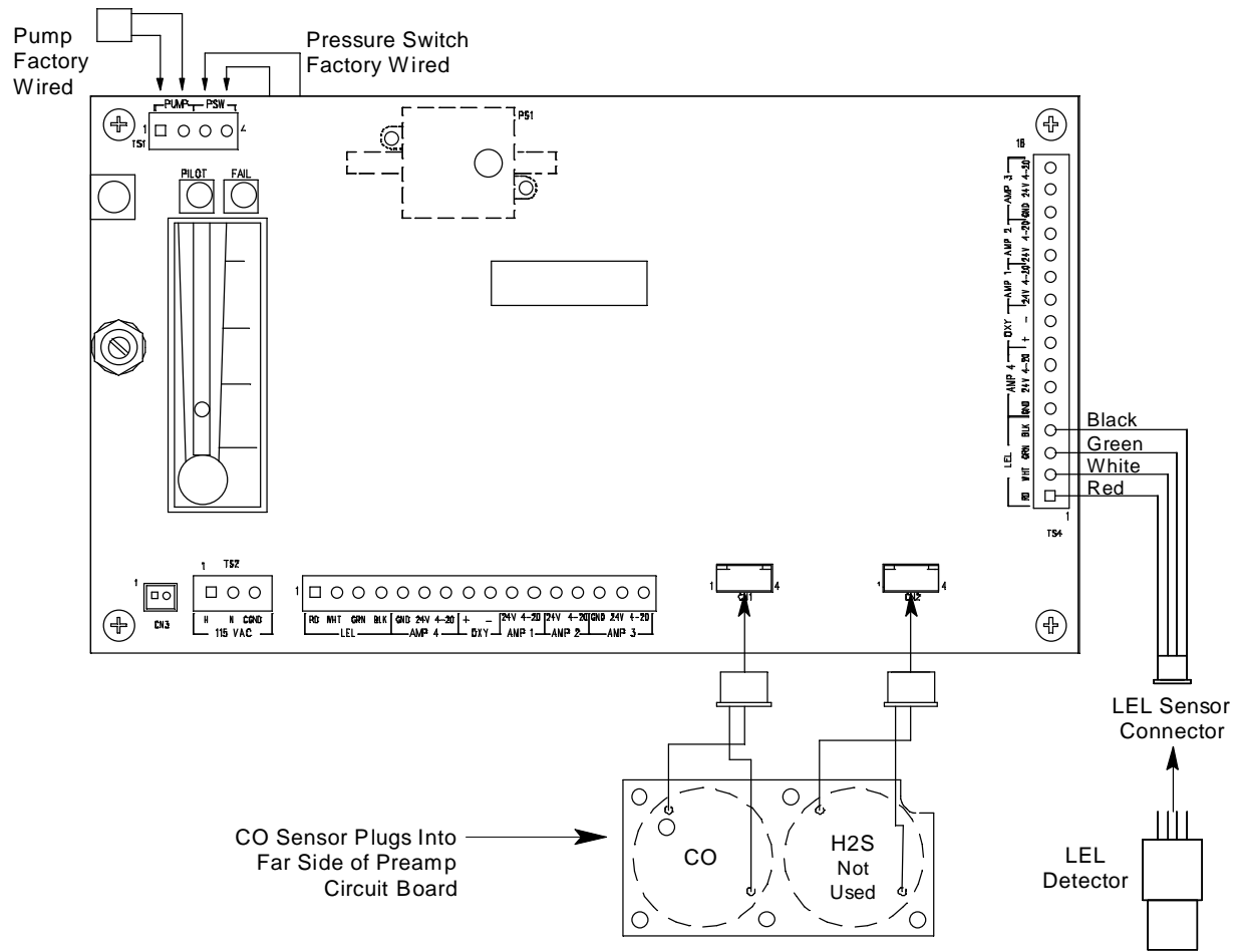
Figure 6: Internal (Factory) Wiring, Sample Draw Detector
