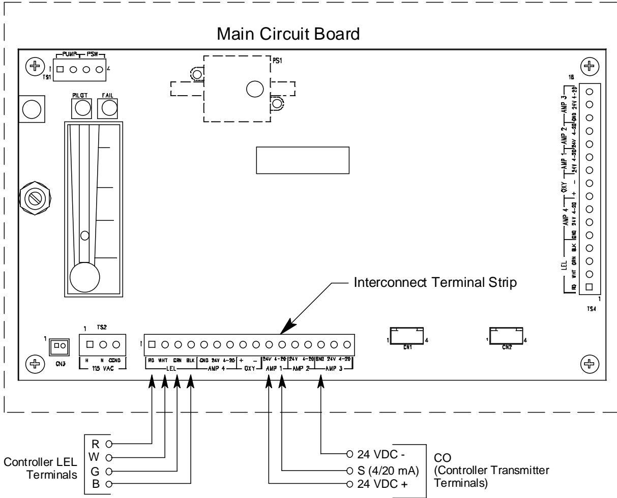
Figure 5: External (Field) Wiring, Sample Draw Detector
