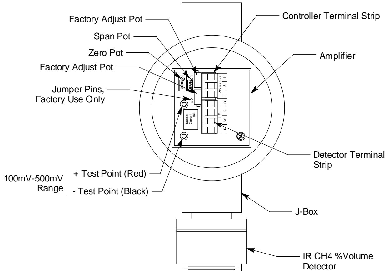
Figure 1: Methane Transmitter Component Location
