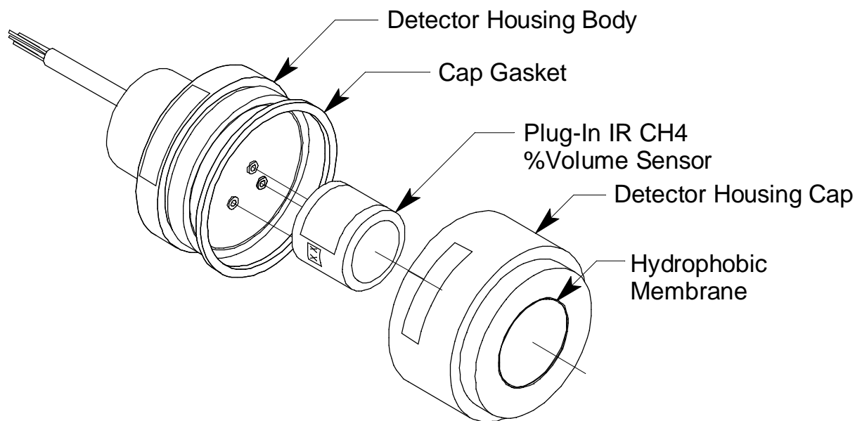
Figure 2: Infrared CH 4 %Vol. Detector Component Location
