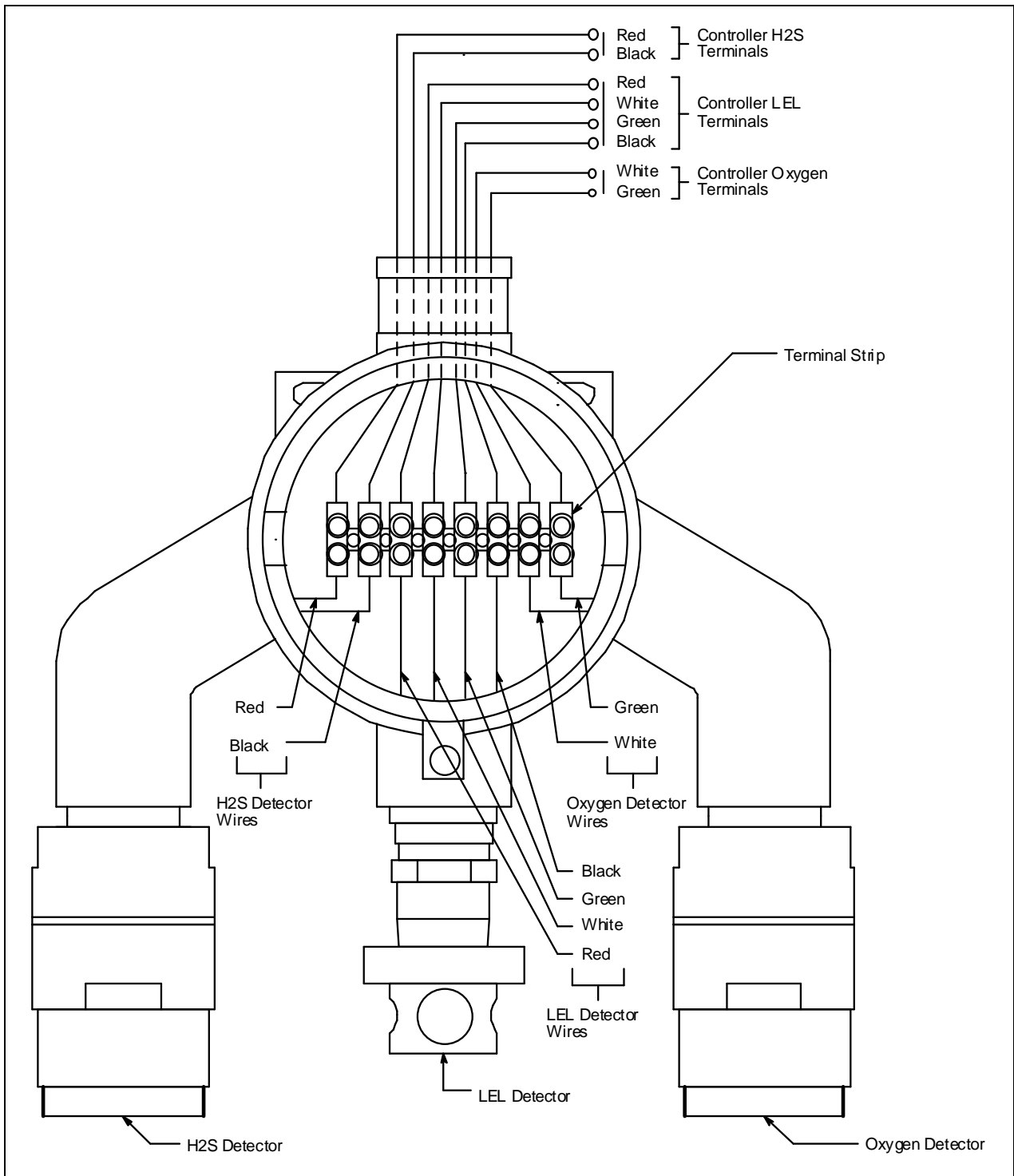
Figure 20: Wiring a 65-2480RK-51 to a Controller
