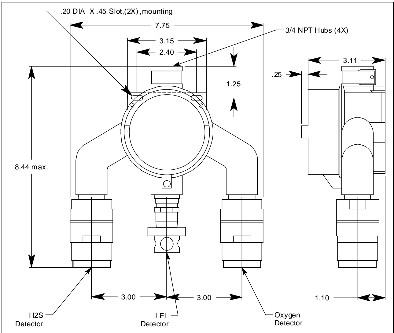
Figure 11: Outline and Mounting Dimensions 65-2480RK-51
