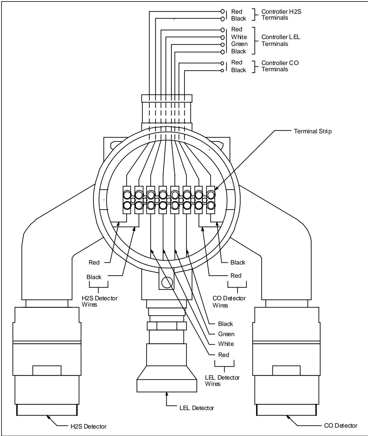
Figure 19: Wiring a 65-2480RK-05 to a Controller
