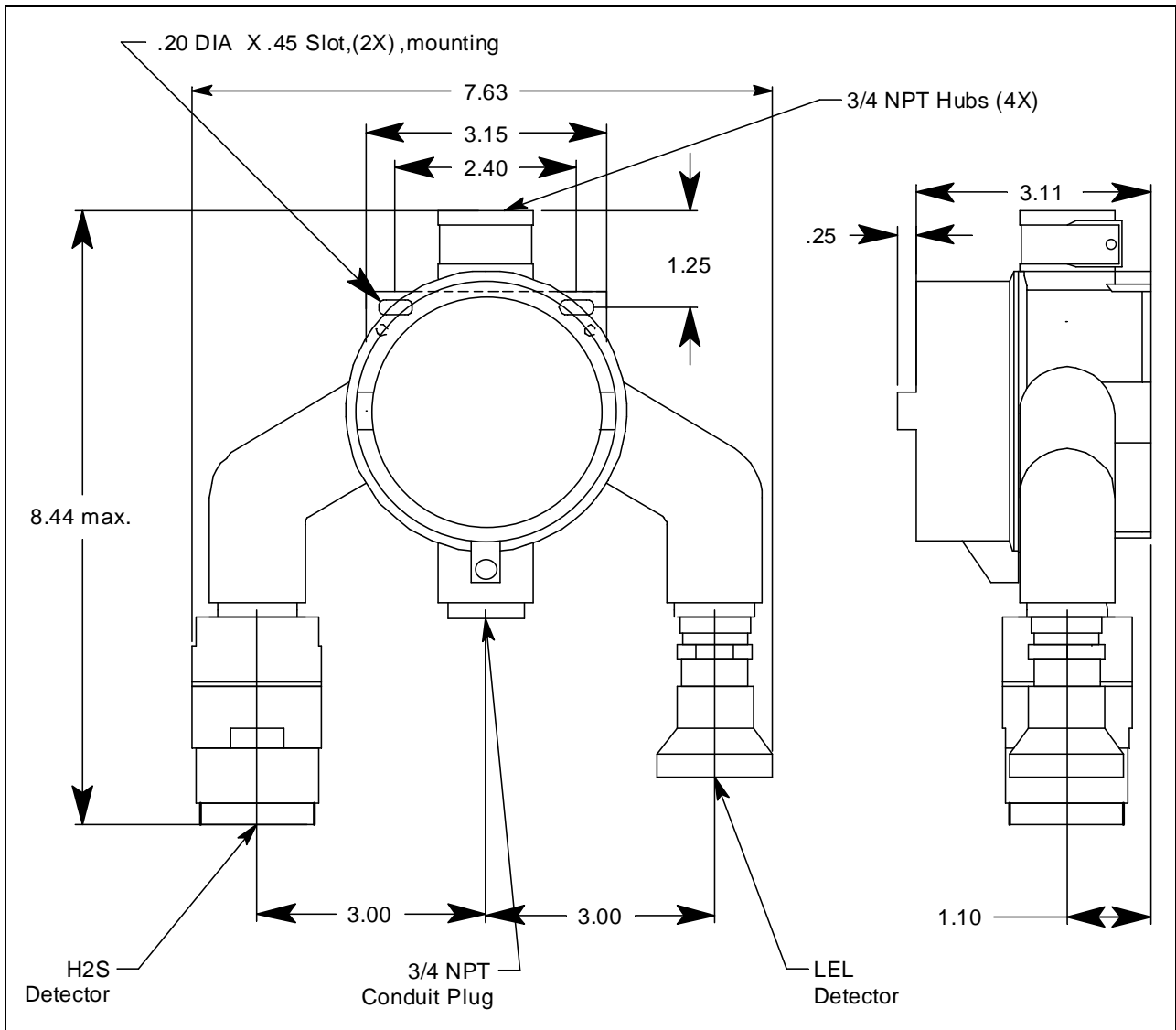
Figure 8: Outline and Mounting Dimensions 65-2480RK-03
