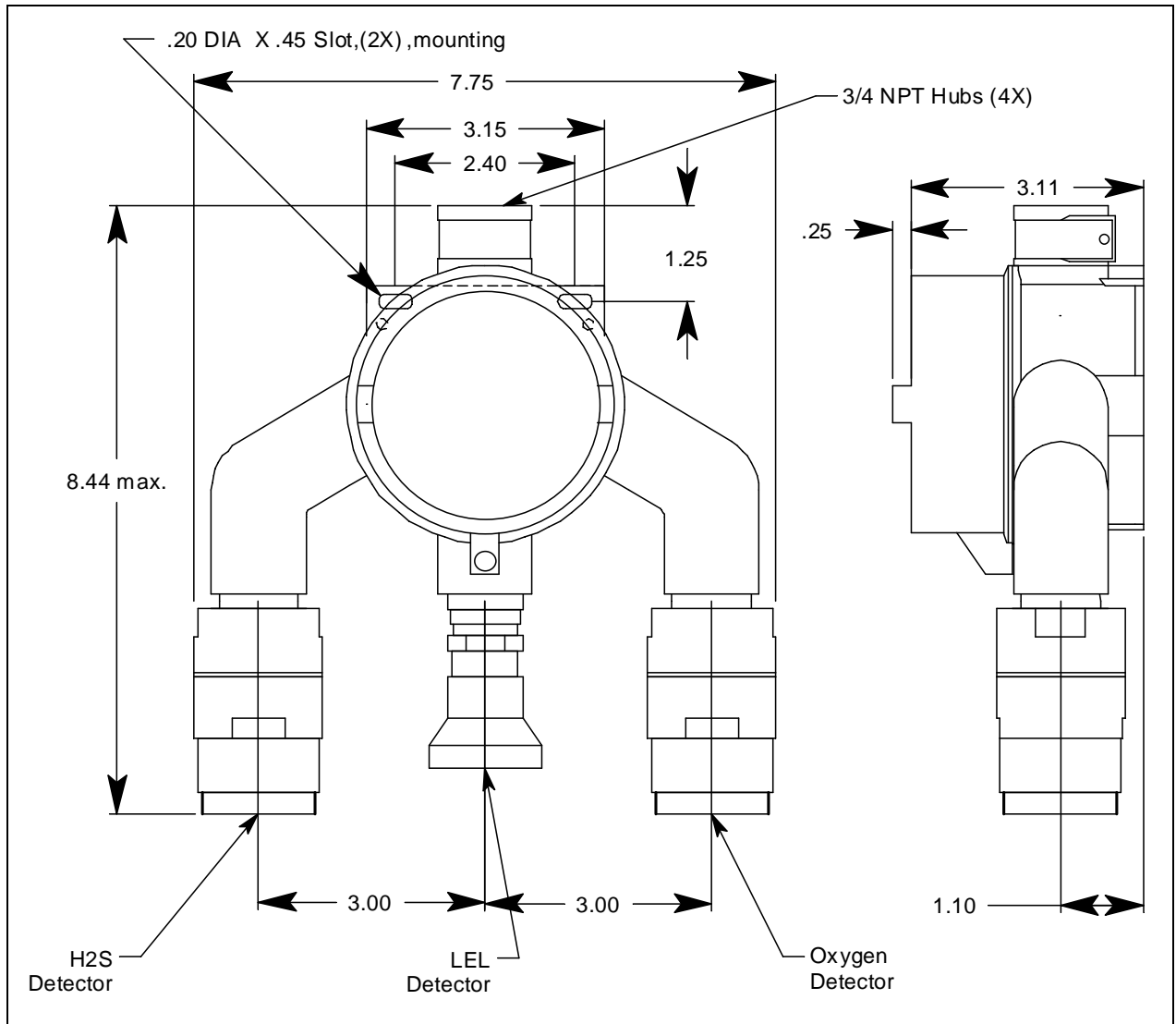
Figure 6: Outline & Mounting Dimensions 65-2480RK-01
