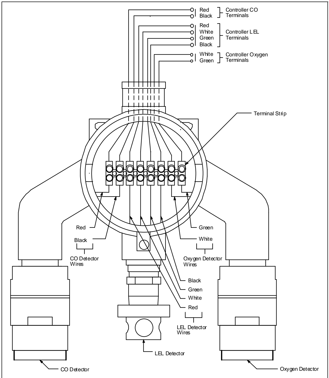
Figure 21: Wiring a 65-2480RK-52 to a Controller
