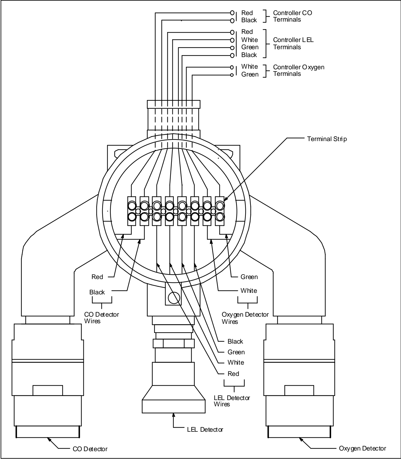
Figure 16: Wiring a 65-2480RK-02 to a Controller
