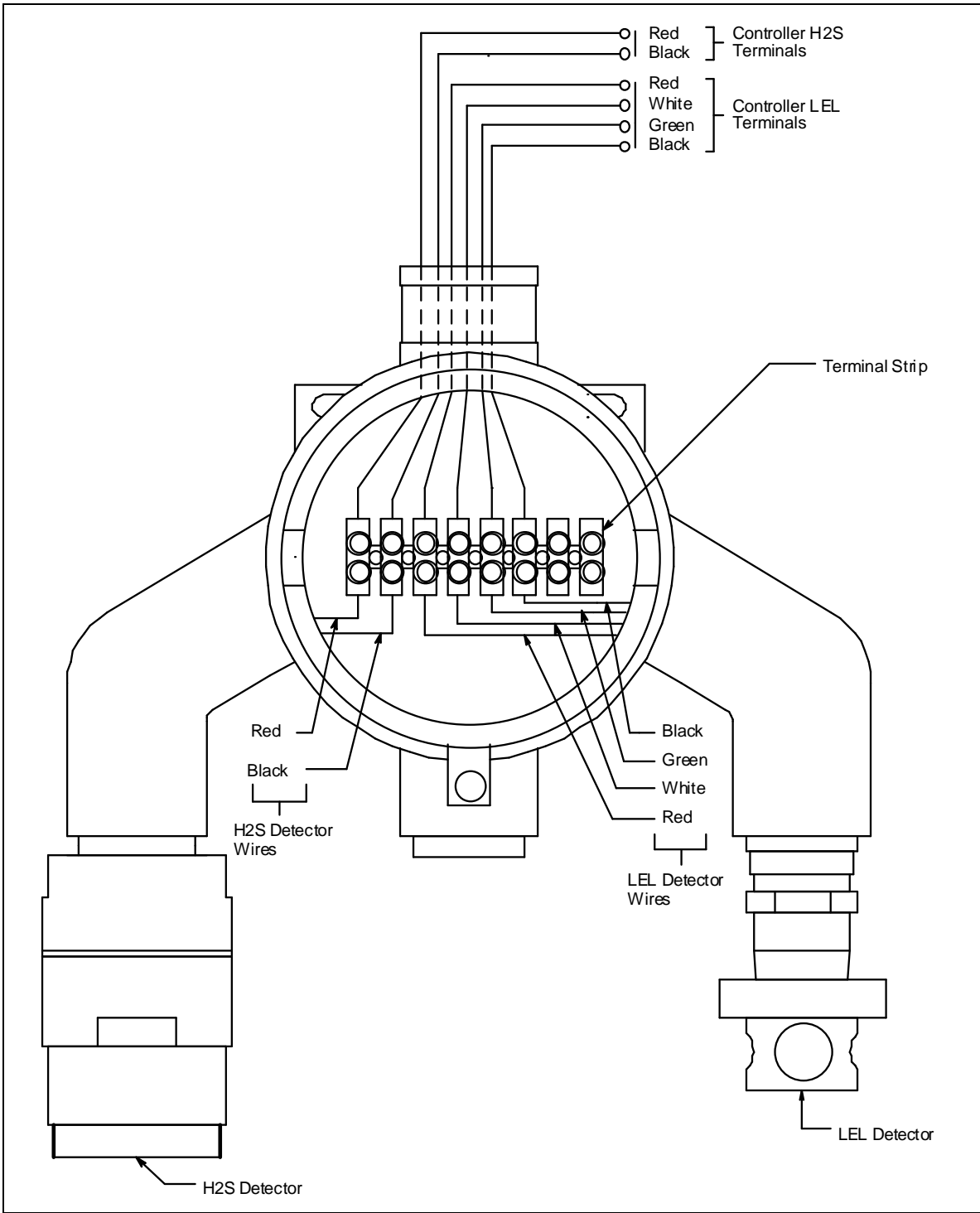
Figure 22: Wiring a 65-2480RK-53 to a Controller
