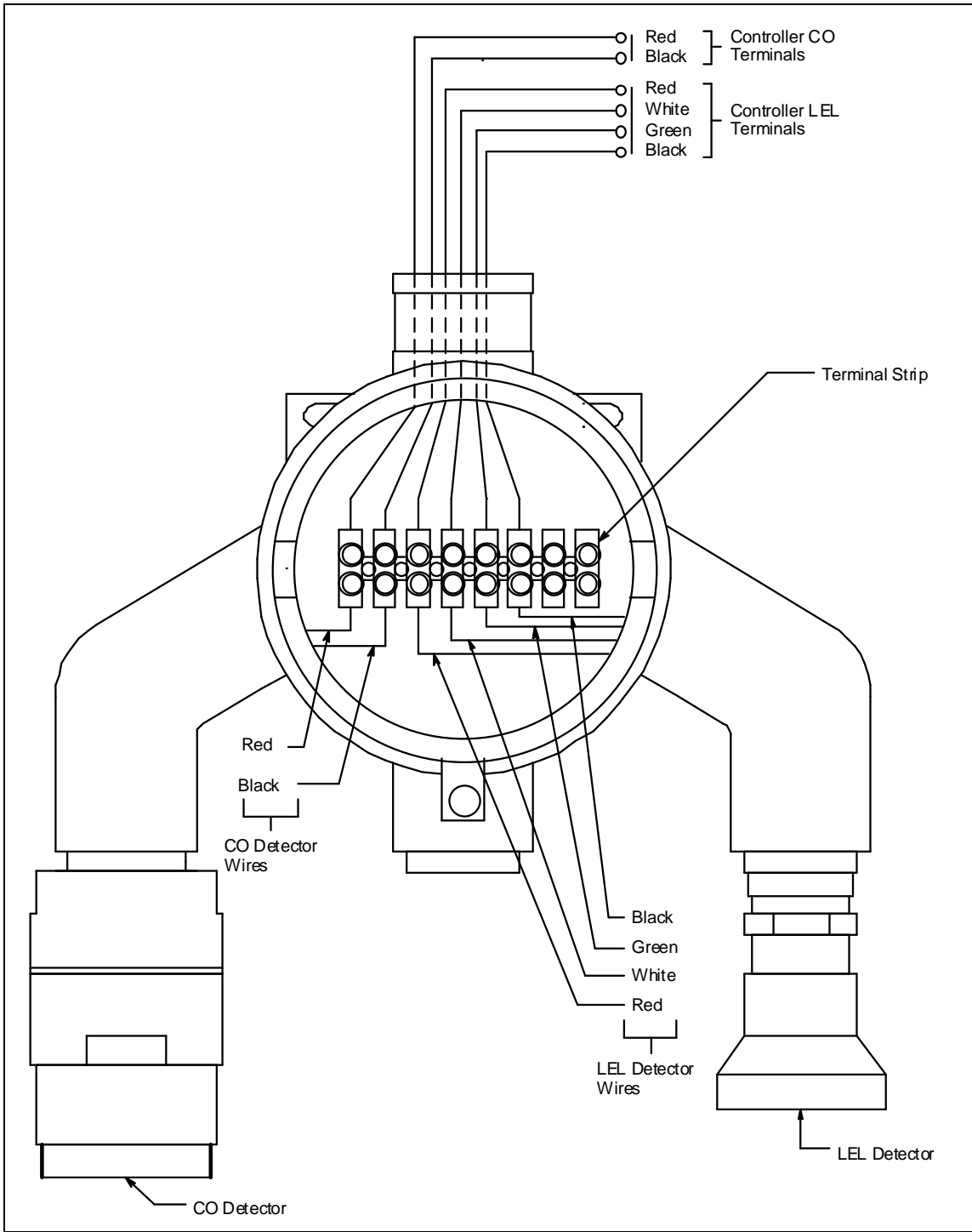
Figure 18: Wiring a 65-2480RK-04 to a Controller
