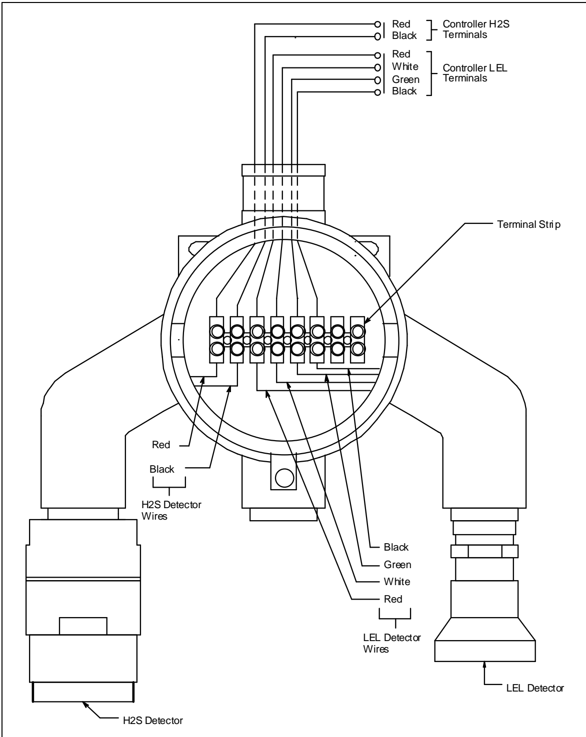
Figure 17: Wiring a 65-2480RK-03 to a Controller
