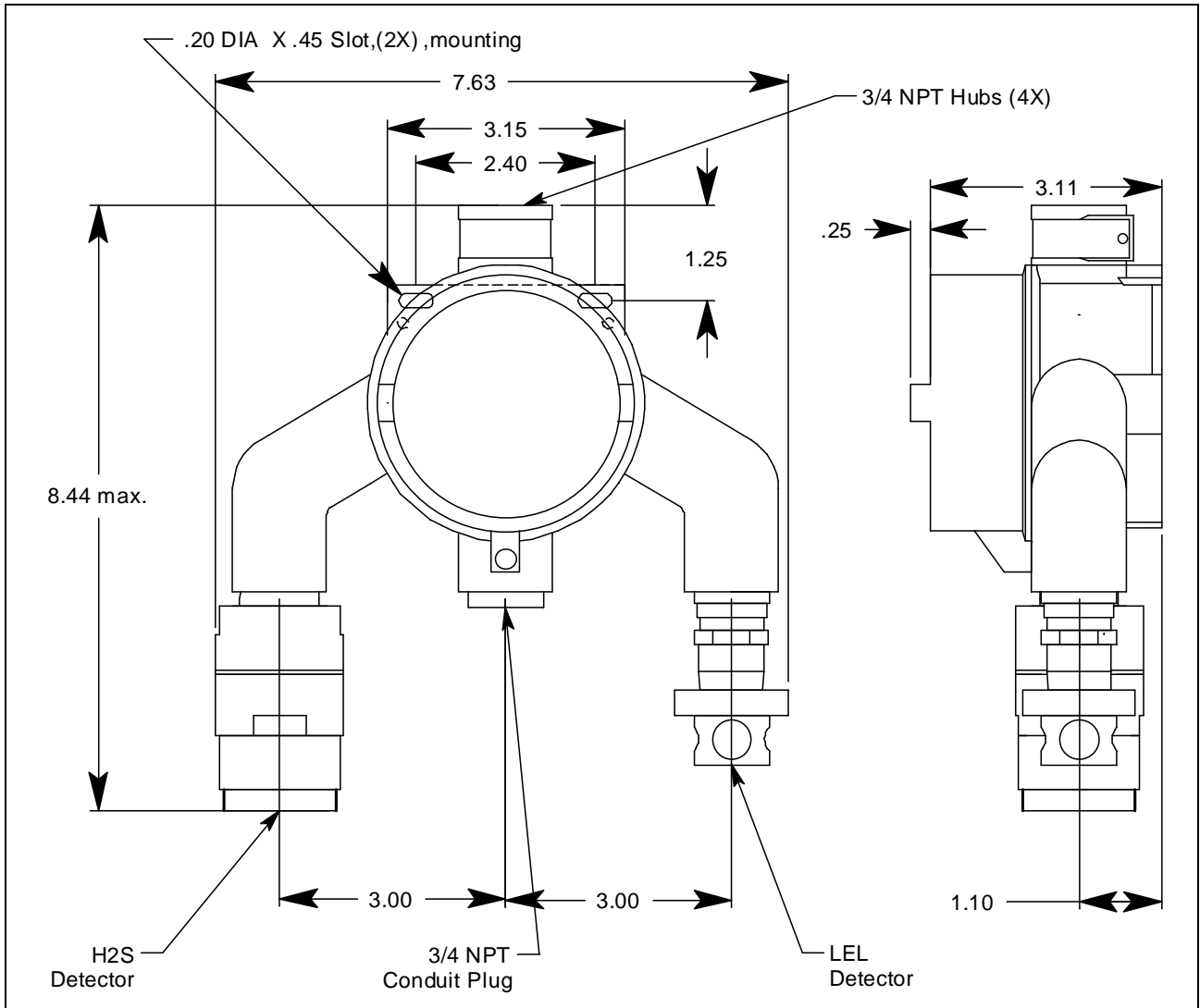
Figure 13: Outline and Mounting Dimensions 65-2480RK-53
