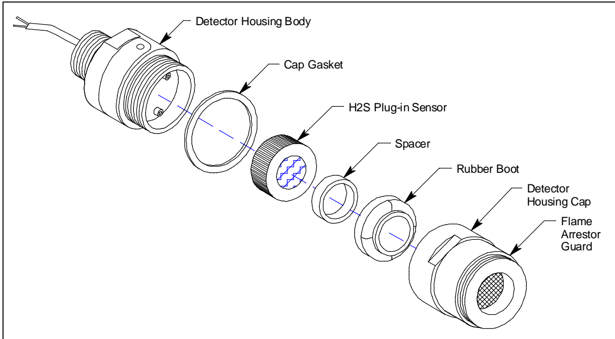
Figure 5: H 2 S Detector Component Location
