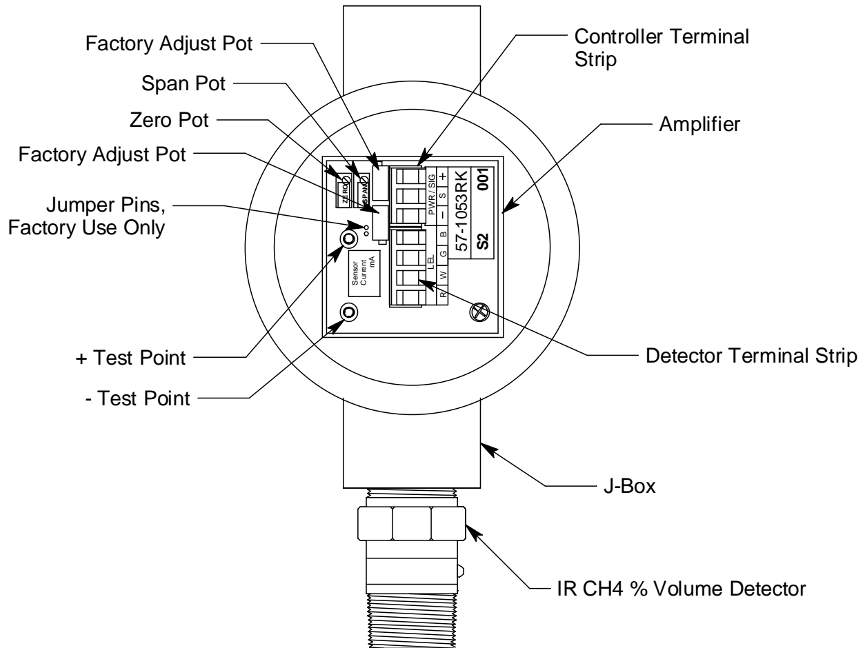
Figure 1: Methane Transmitter Component Location
