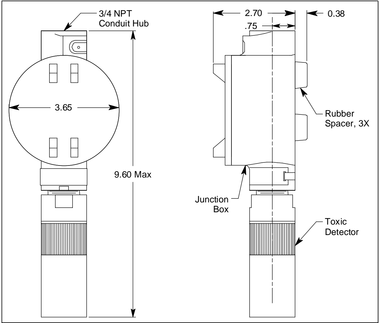
Figure 4: Mounting the Toxic Gas Transmitter
