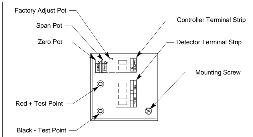
Figure 3: Amplifier Component Location
