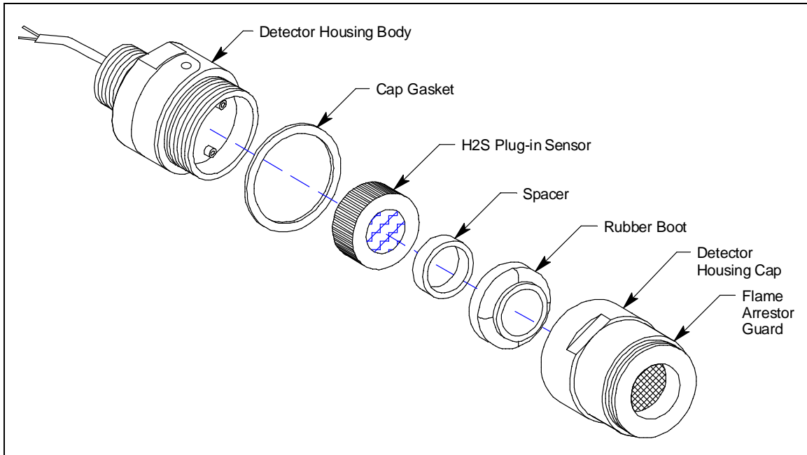
Figure 1: H 2 S Detector Component Location
