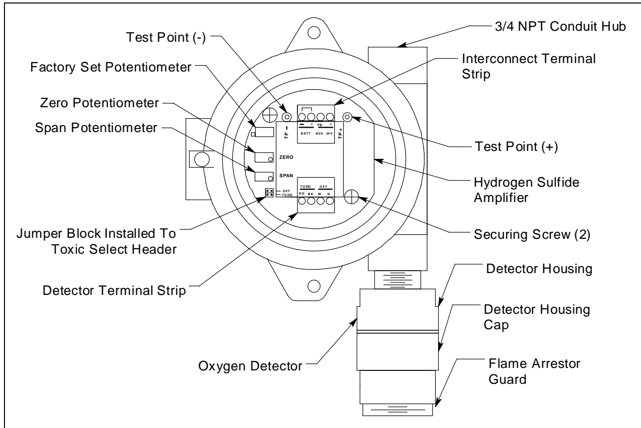
Figure 1: Oxygen Transmitter Component Location
