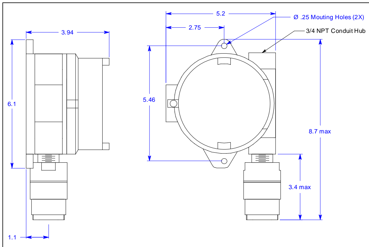
Figure 2: Mounting the Oxygen Transmitter
