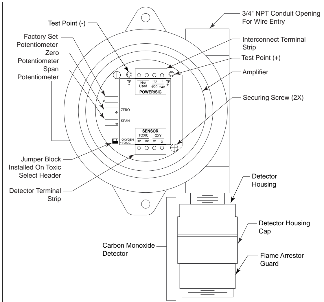
Figure 1: CO Transmitter Component Location
