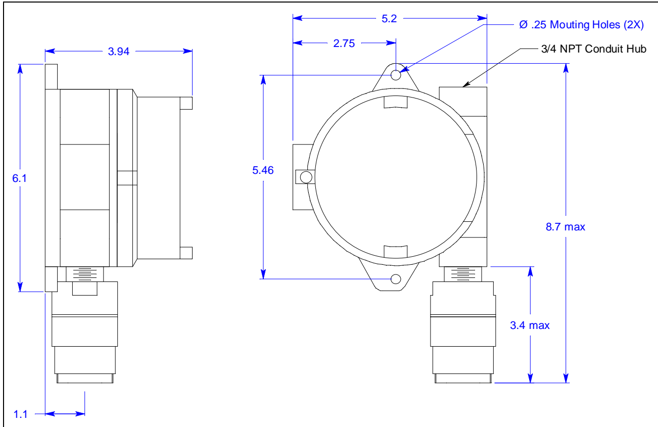
Figure 2: Mounting the CO Transmitter
