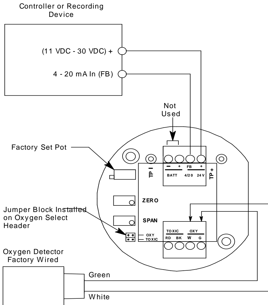
Figure 3: Wiring the Oxygen Transmitter to a Controller
