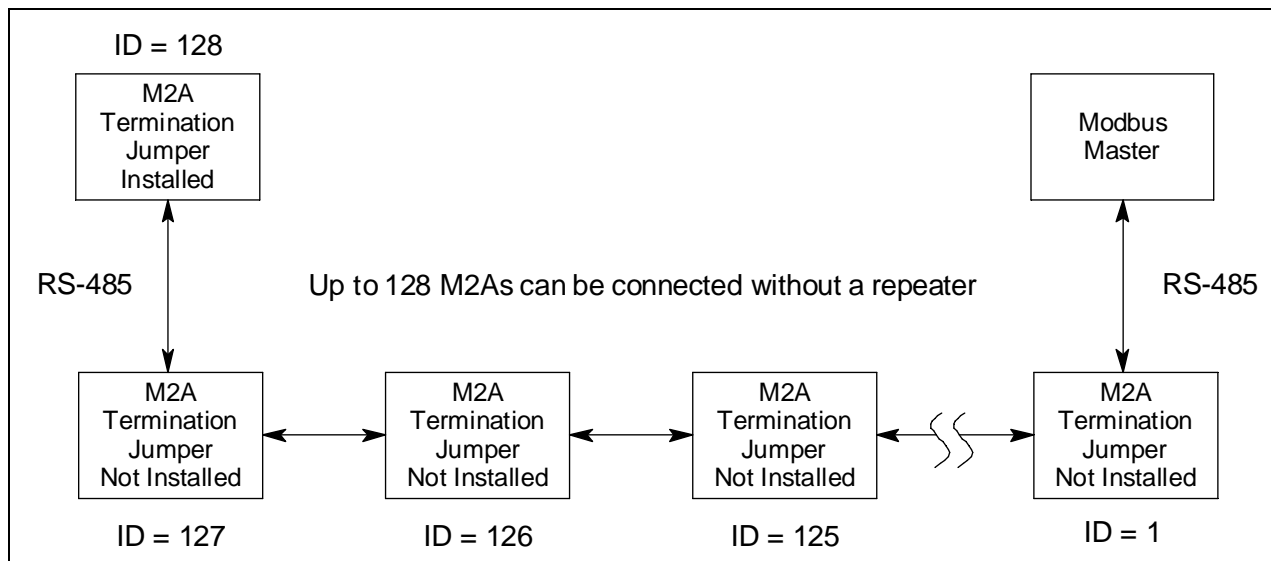
Figure 13: Multiple M2A-XLs in a Daisy Chain Configuration
