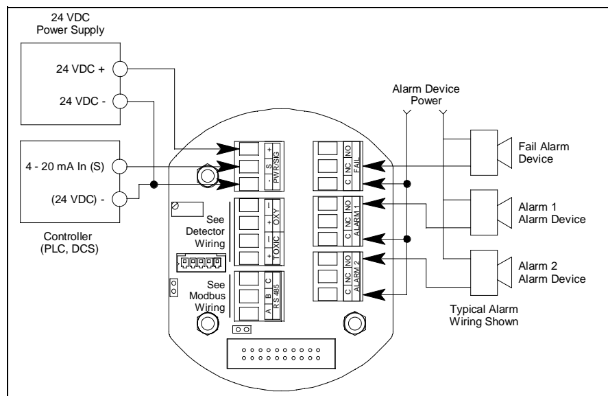
Figure 15: PLC and DCS Device Wiring
