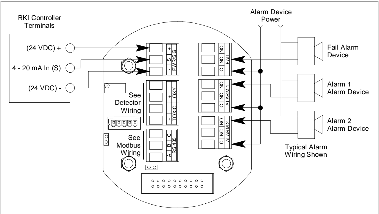
Figure 9: Wiring the M2A to a Controller and Alarm Devices
