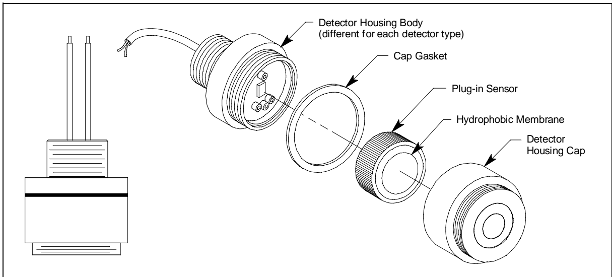
Figure 2: Detector Component Location
