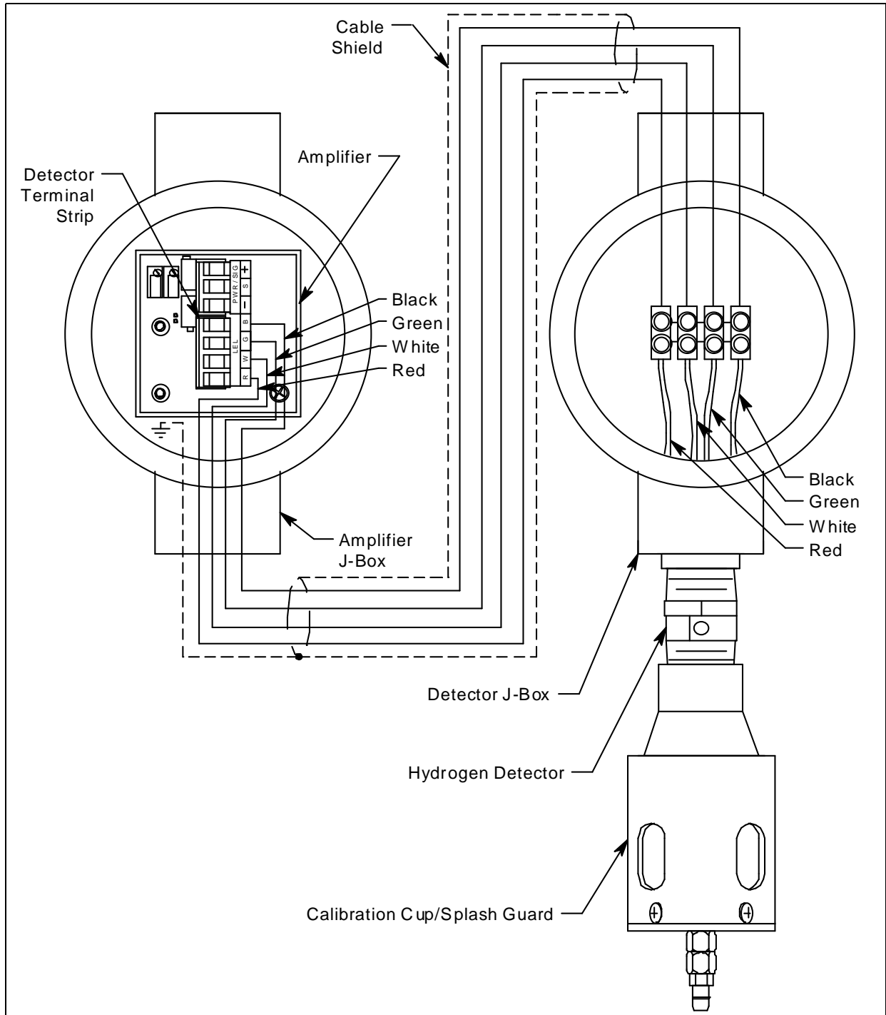
Figure 4: Wiring the Detector to the Amplifier
