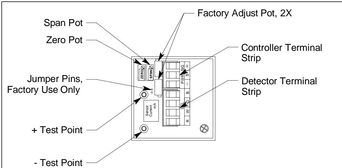
Figure 2: Amplifier Component Location
