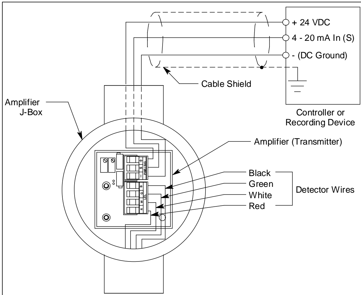
Figure 5: Wiring the Amplifier to a Controller
