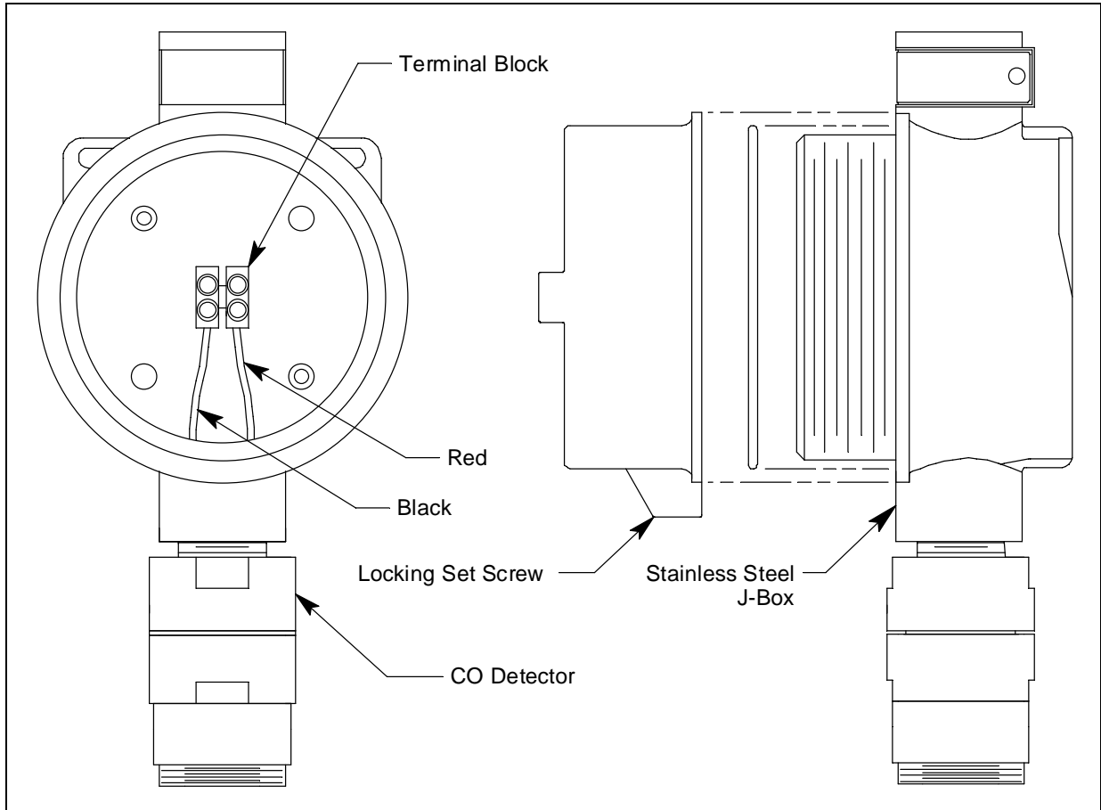
Figure 1: CO Detector Component Location
