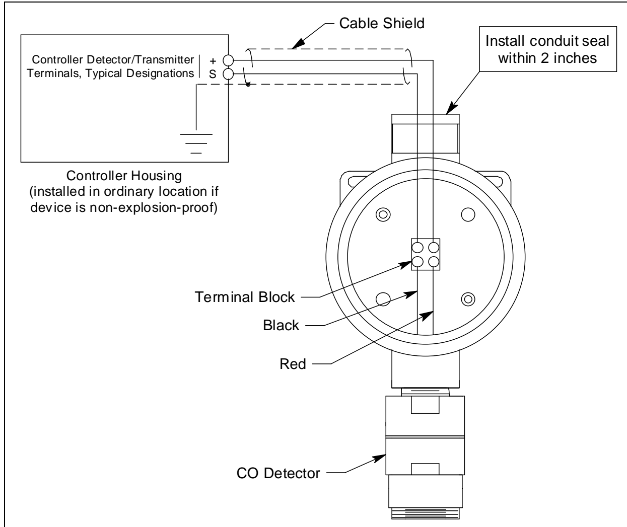
Figure 4: Wiring the CO Detector to a Controller
