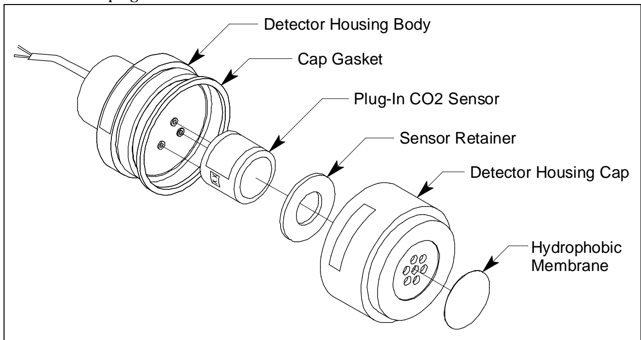
Figure 2: CO 2 Detector Component Location
