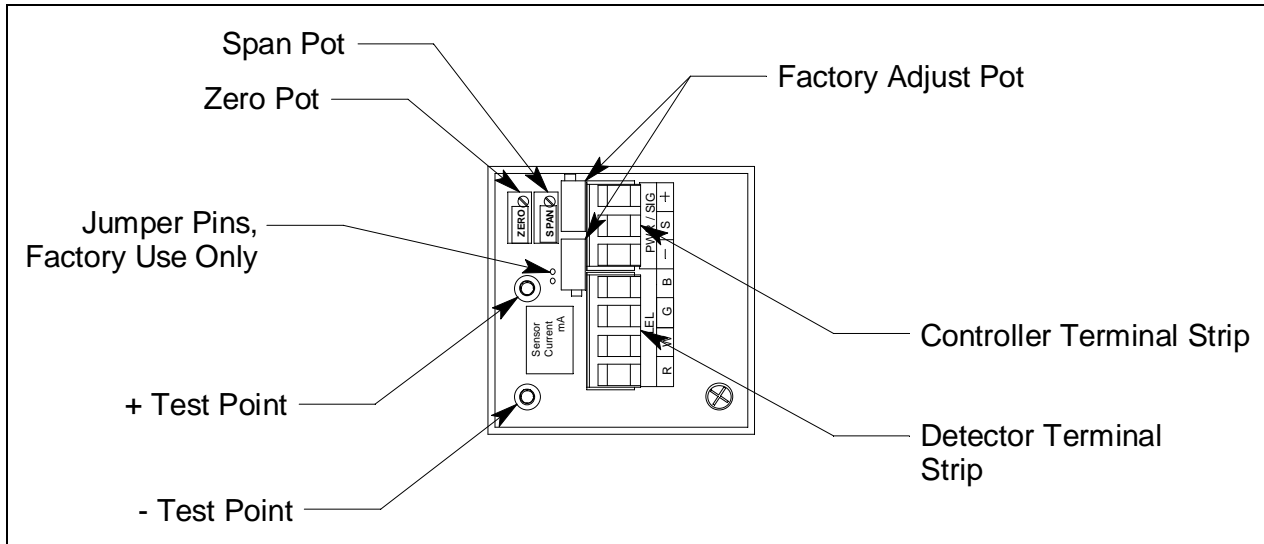
Figure 3: Amplifier Component Location
