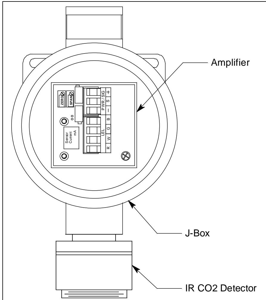
Figure 1: CO 2 Transmitter Component Location
