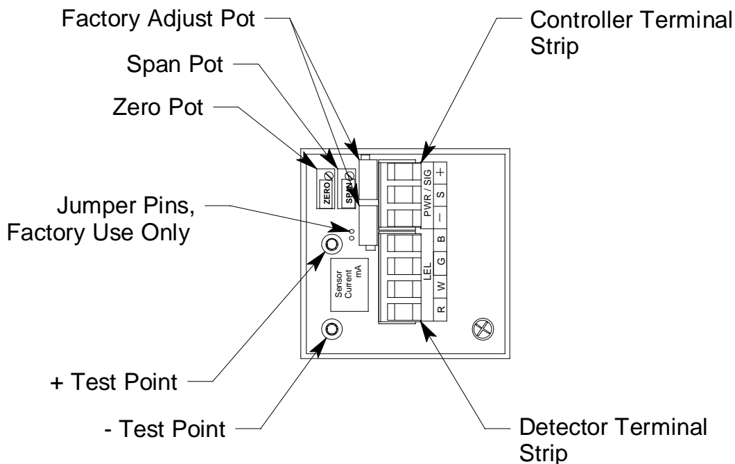
Figure 2: Amplifier Component Location
