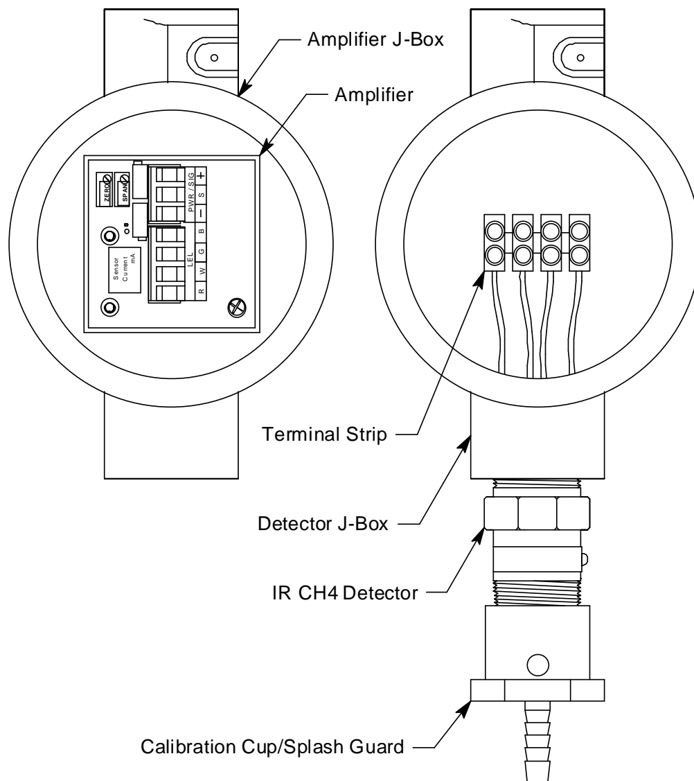
Figure 1: Methane Transmitter Component Location
