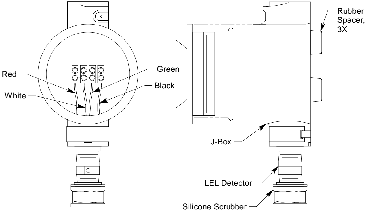
Figure 1: 61-1000RK-SI Component Location
