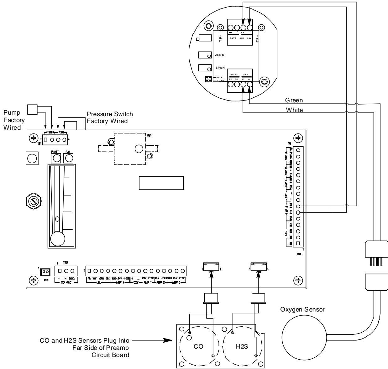
Figure 7: Internal (Factory) Wiring
