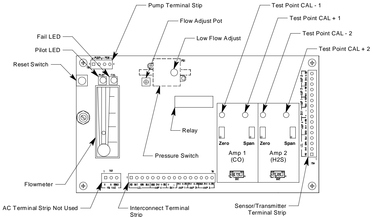
Figure 4: Main Circuit Board
