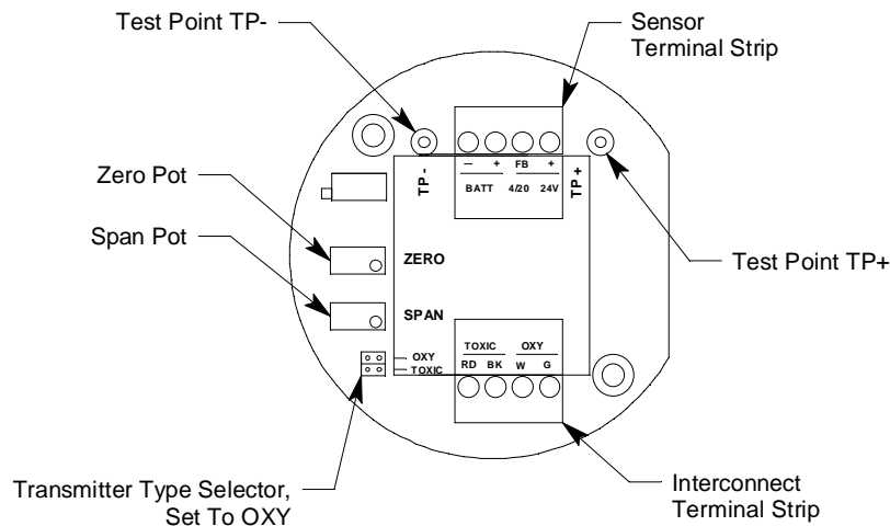
Figure 3: Oxygen Transmitter
