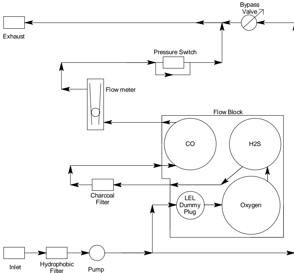
Figure 2: Sample-Draw Detector Flow Diagram
