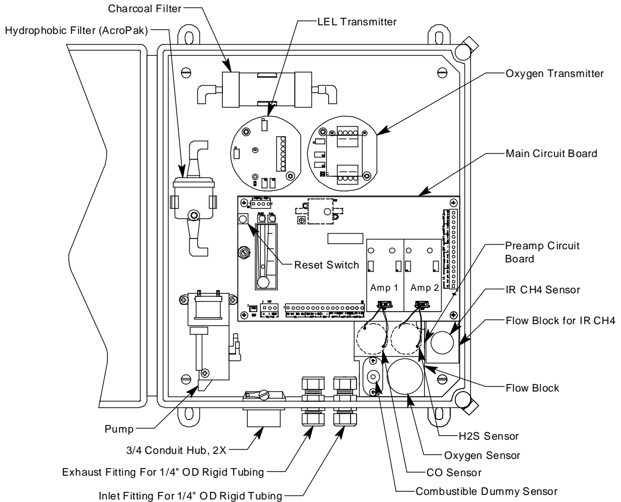
Figure 1: Sample-Draw Detector Component Location
