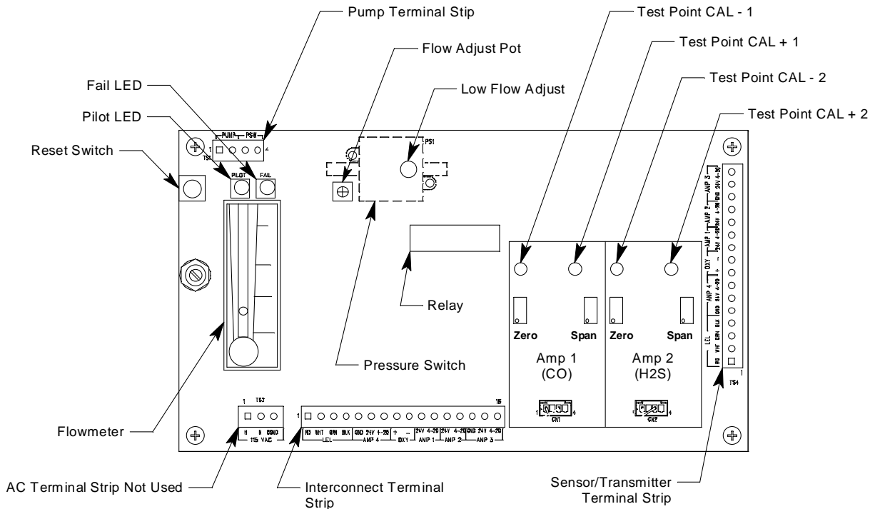
Figure 5: Main Circuit Board
