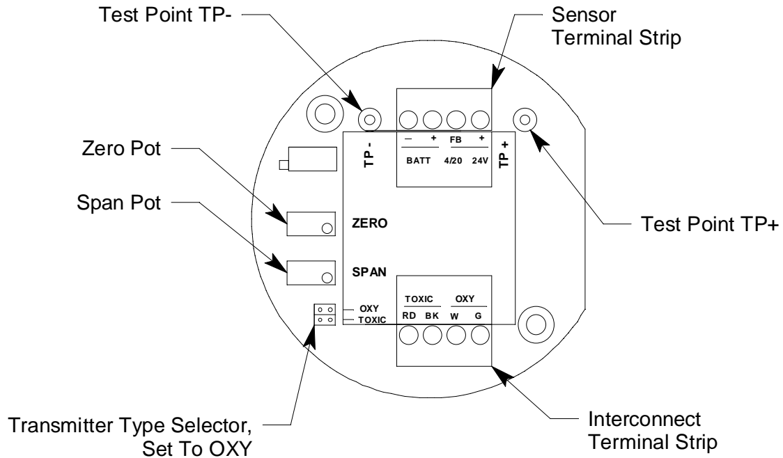
Figure 4: Oxygen Transmitter
