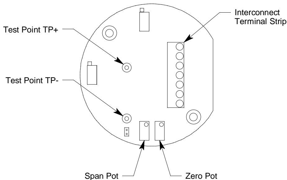
Figure 3: LEL Transmitter
