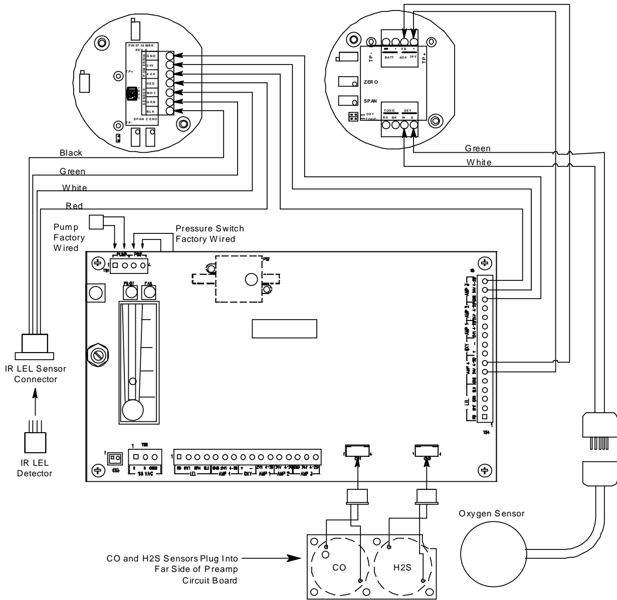
Figure 8: Internal (Factory) Wiring
