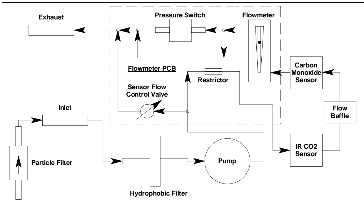
Figure 2: Flow Diagram
