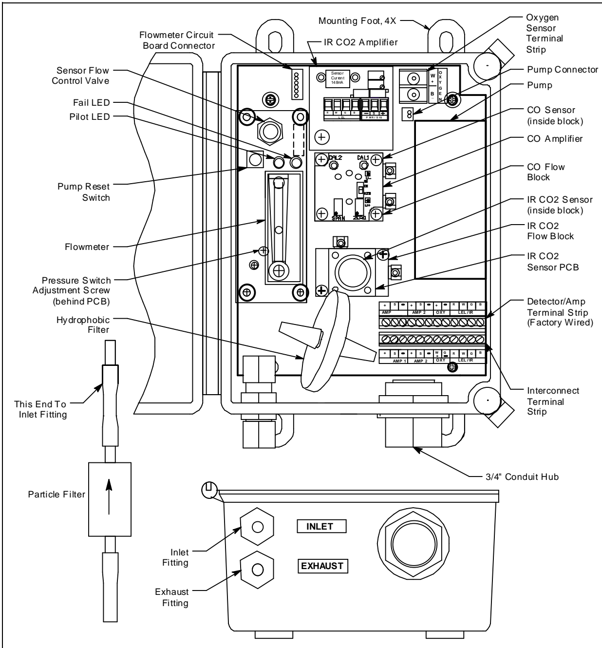
Figure 1: Component Location
