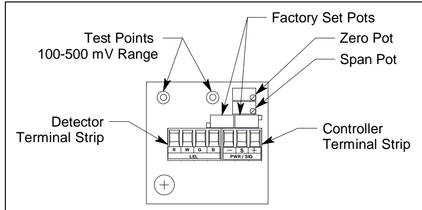
Figure 3: IR CO 2 Amplifier Component Location
