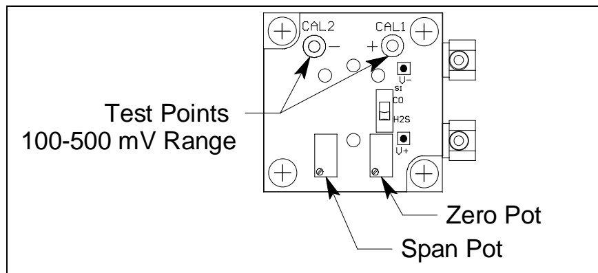
Figure 4: CO Amplifier Component Location
