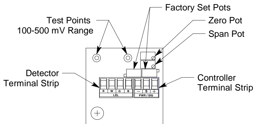
Figure 3: IR CO 2 Amplifier Component Location
