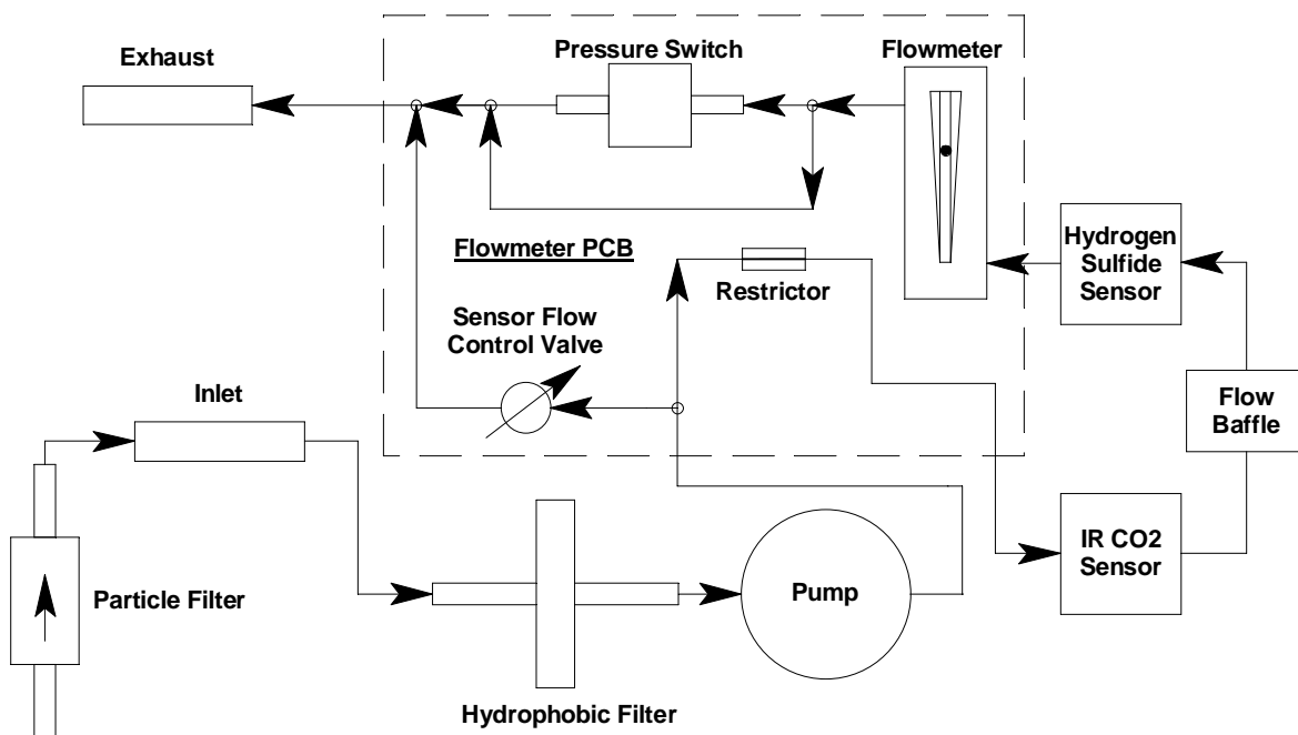
Figure 2: Carbon Dioxide/Hydrogen Sulfide Sample-Draw Detector Flow Diagram
