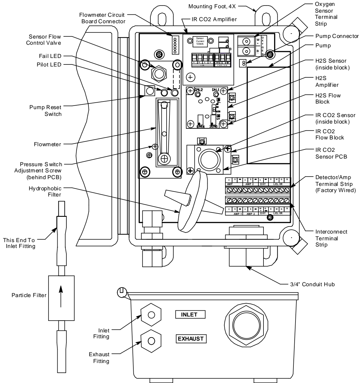
Figure 1: Carbon Dioxide/Hydrogen Sulfide Sample-Draw Detector Component Location
