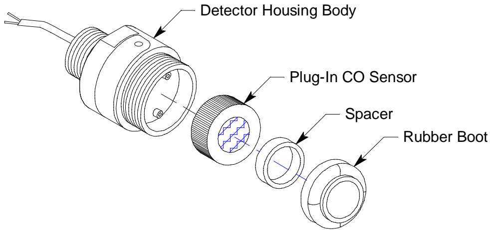
Figure 3: CO Detector Component Location
