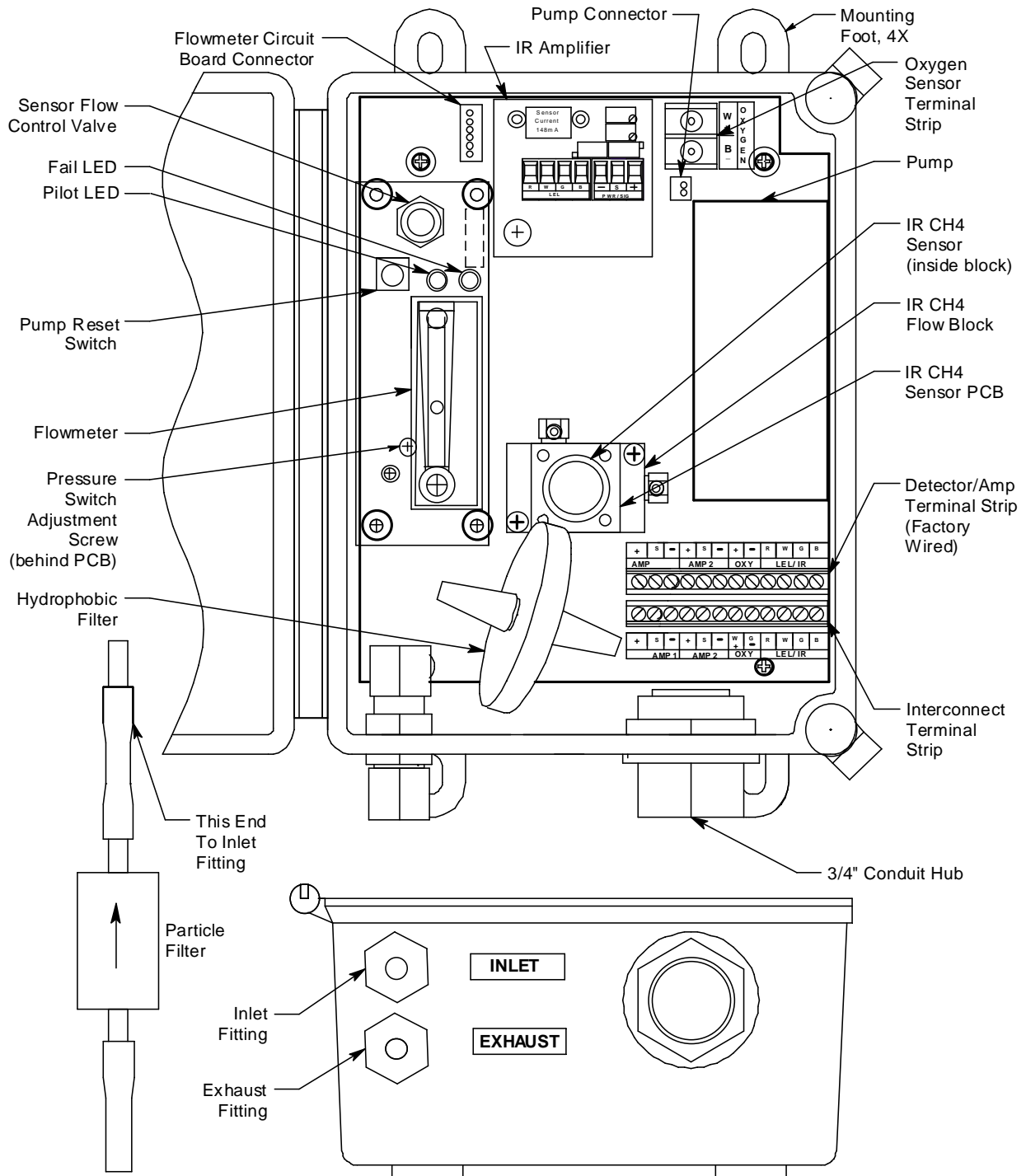
Figure 1: Methane Sample-Draw Detector Component Location
