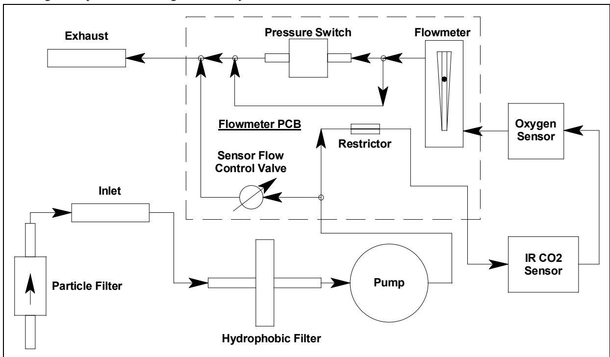
Figure 2: Flow Diagram
