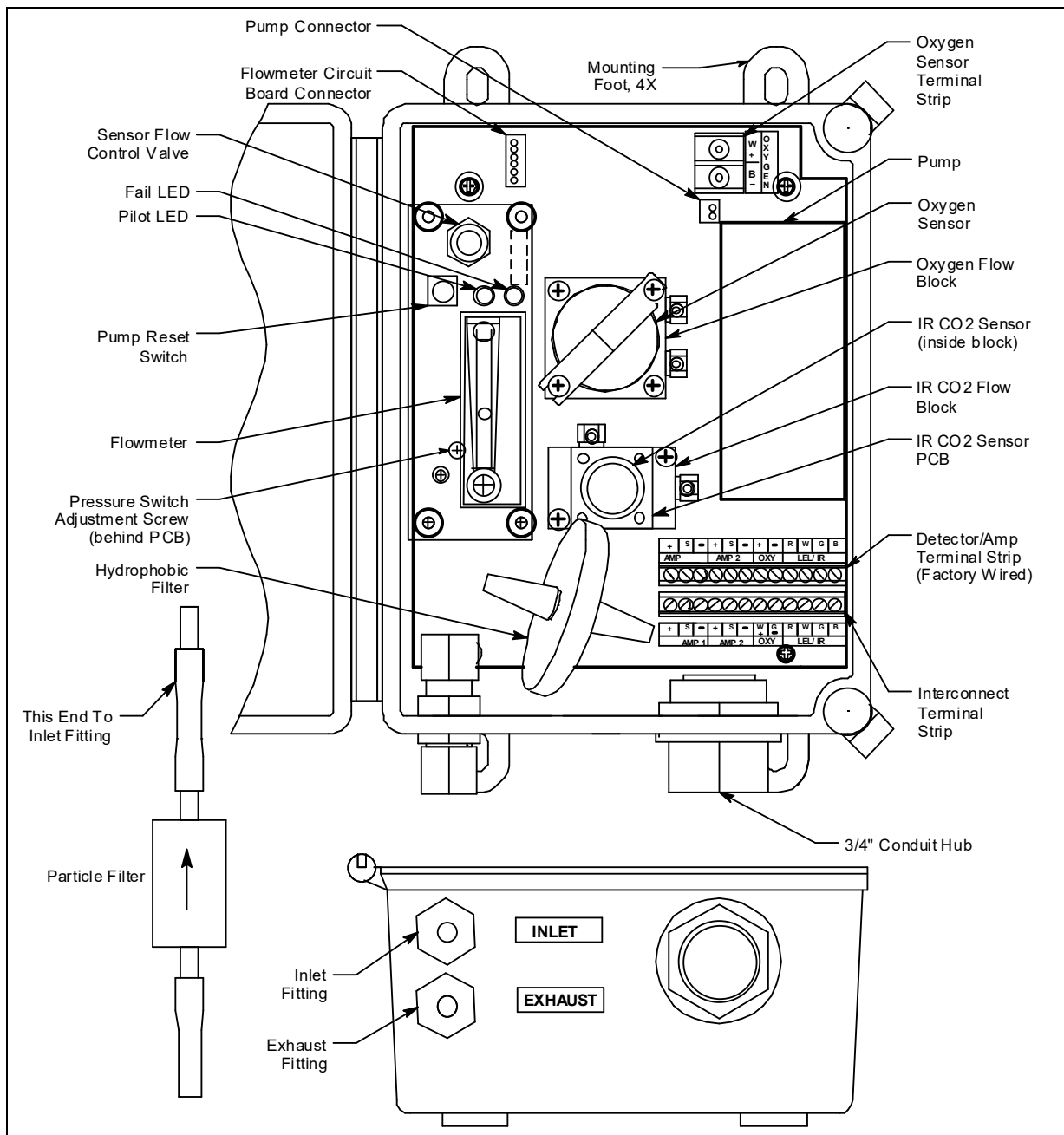
Figure 1: Component Location
