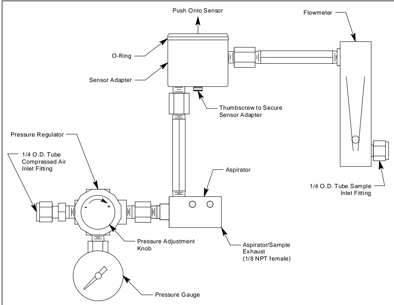
Figure 1: Component Location
