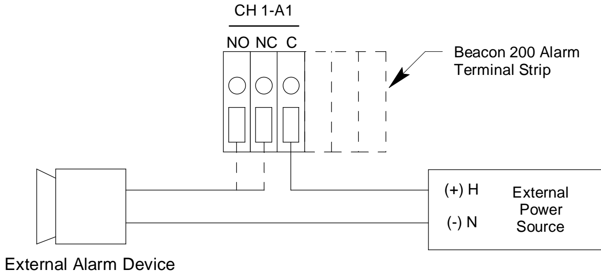
Figure 8. Typical External Alarm Wiring
