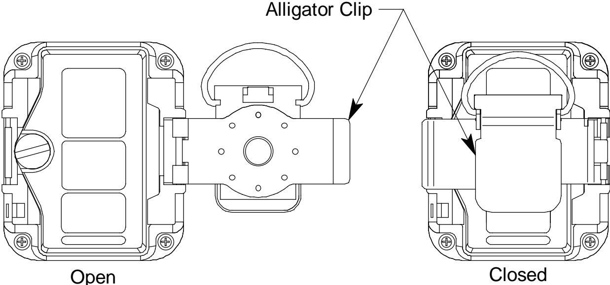
Figure 3: Alligator Clip
