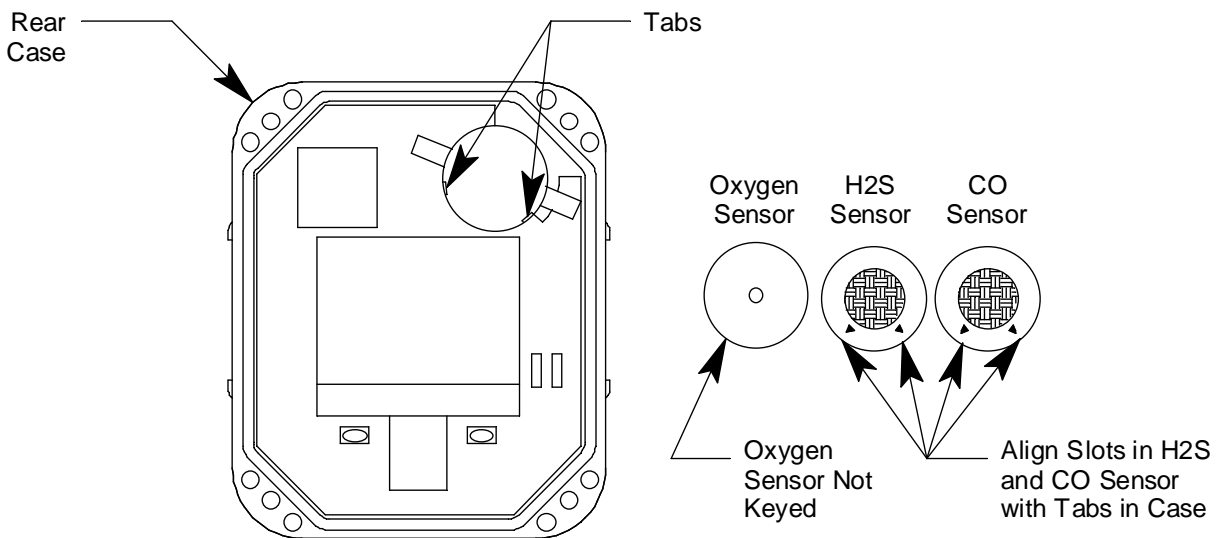
Figure 16: Replacing the Sensor
