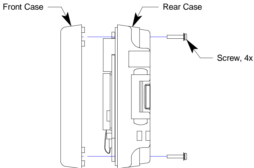
Figure 15: Case Separation
