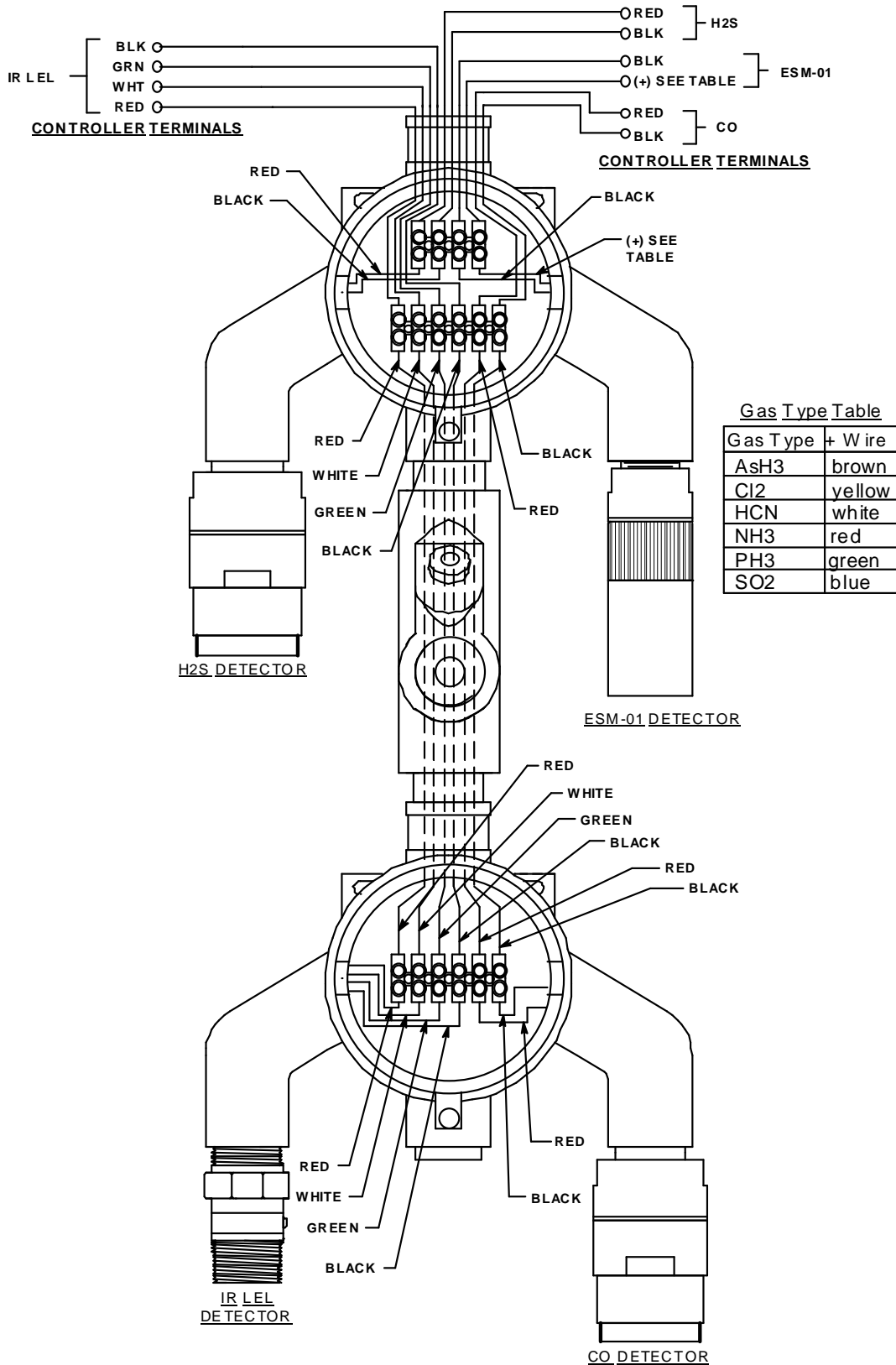
Figure 14: Wiring for IR LEL/CO/H 2 S/ESM-01 Versions (65-2484RK-3X)
