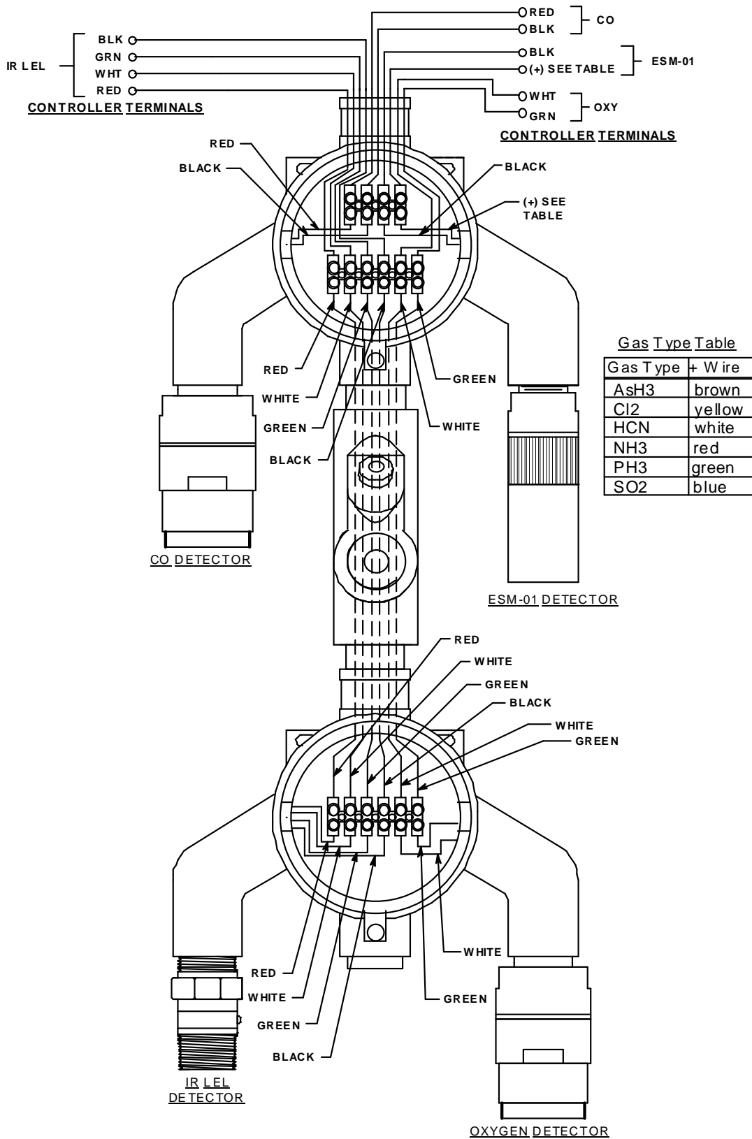
Figure 13: Wiring for IR LEL/O 2 /CO/ESM-01 Versions (65-2484RK-5X)
