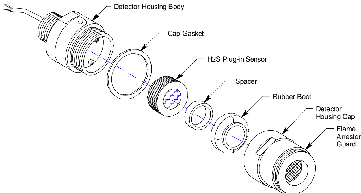
Figure 3: H 2 S Detector Component Location
