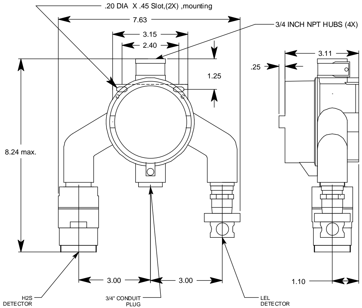
Figure 13: Outline and Mounting Dimensions 65-2480RK-53
