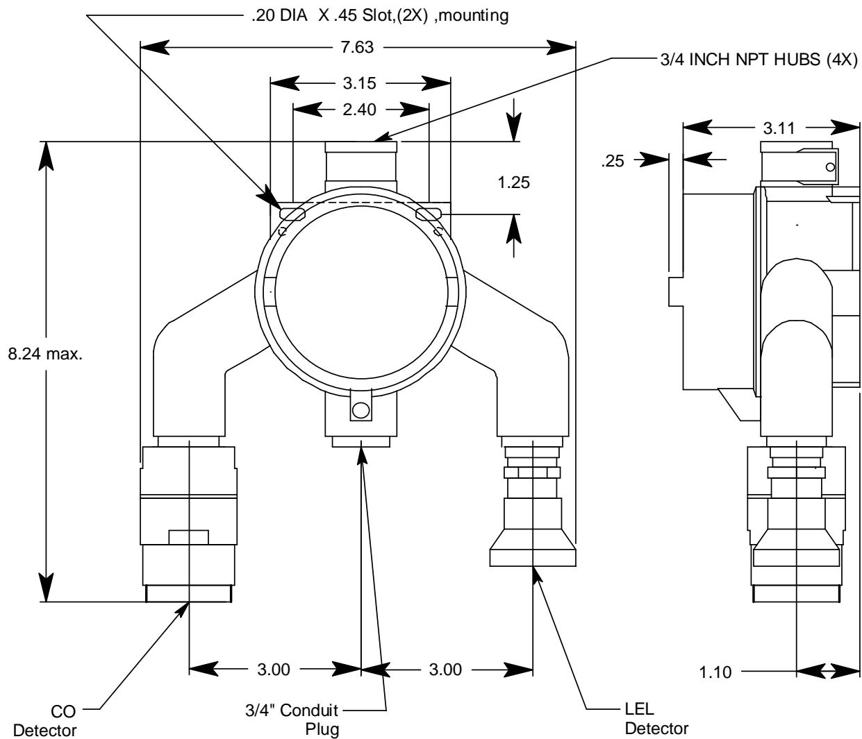
Figure 9: Outline and Mounting Dimensions 65-2480RK-04
