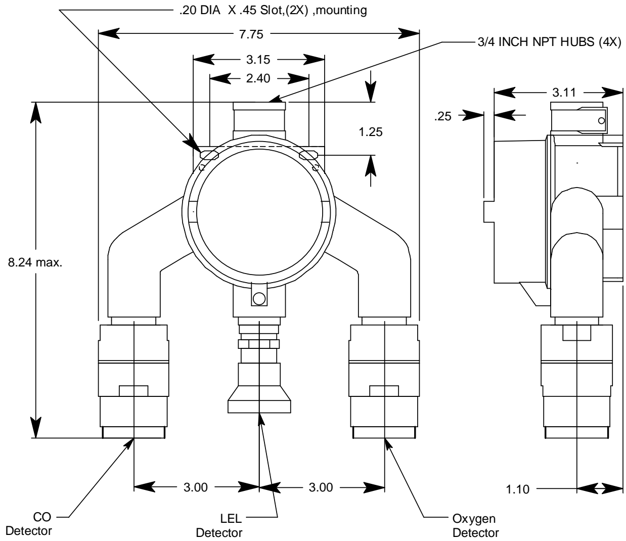
Figure 7: Outline and Mounting Dimensions 65-2480RK-02
