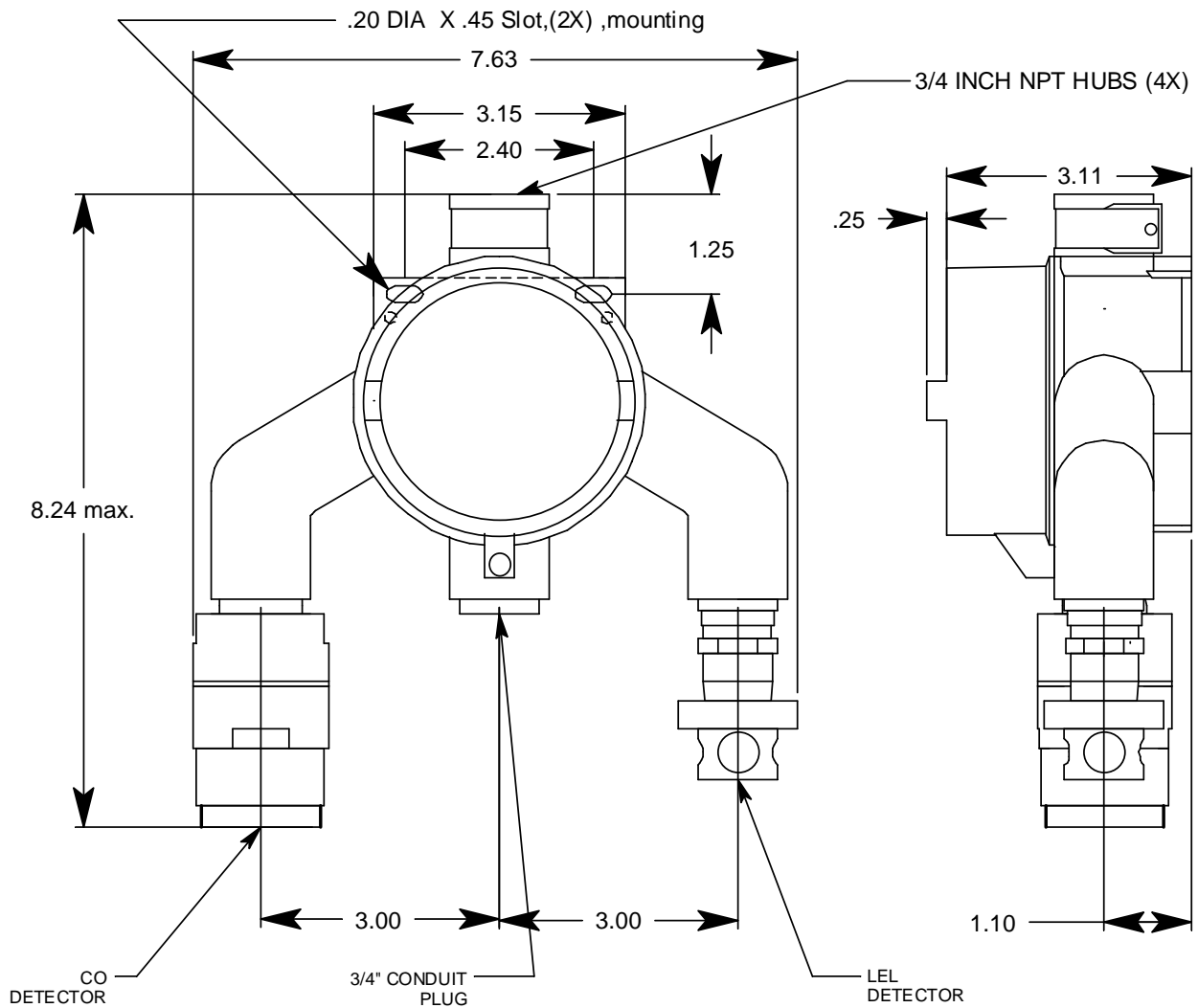
Figure 14: Outline and Mounting Dimensions 65-2480RK-54
