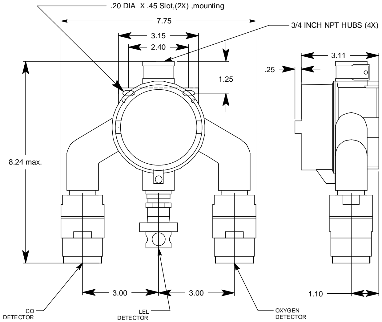
Figure 12: Outline and Mounting Dimensions 65-2480RK-52
