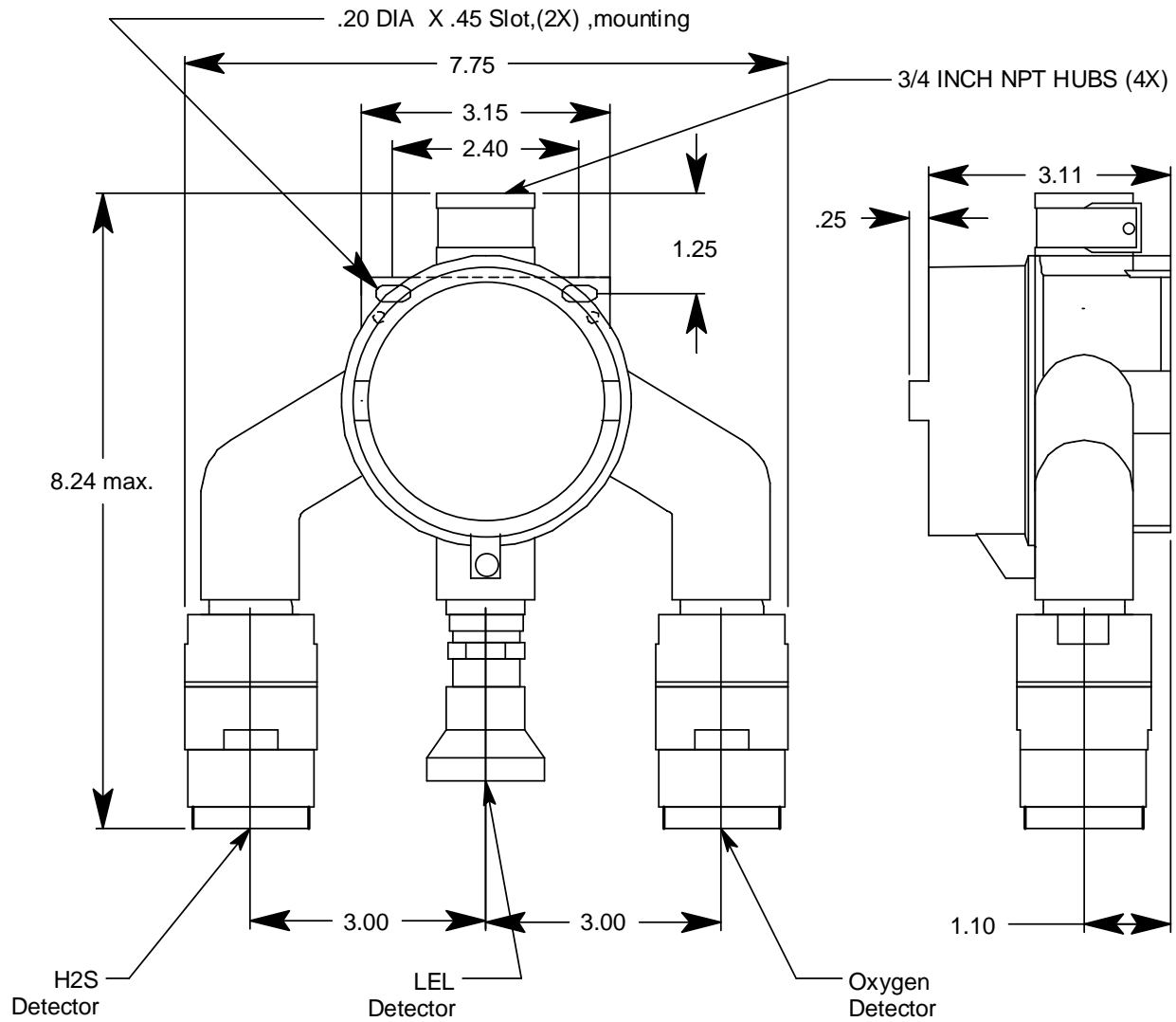
Figure 6: Outline & Mounting Dimensions 65-2480RK-01
