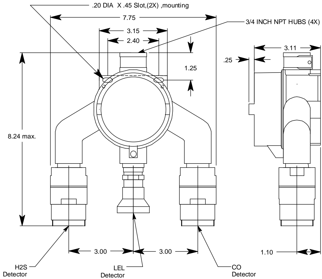
Figure 10: Outline and Mounting Dimensions 65-2480RK-05
