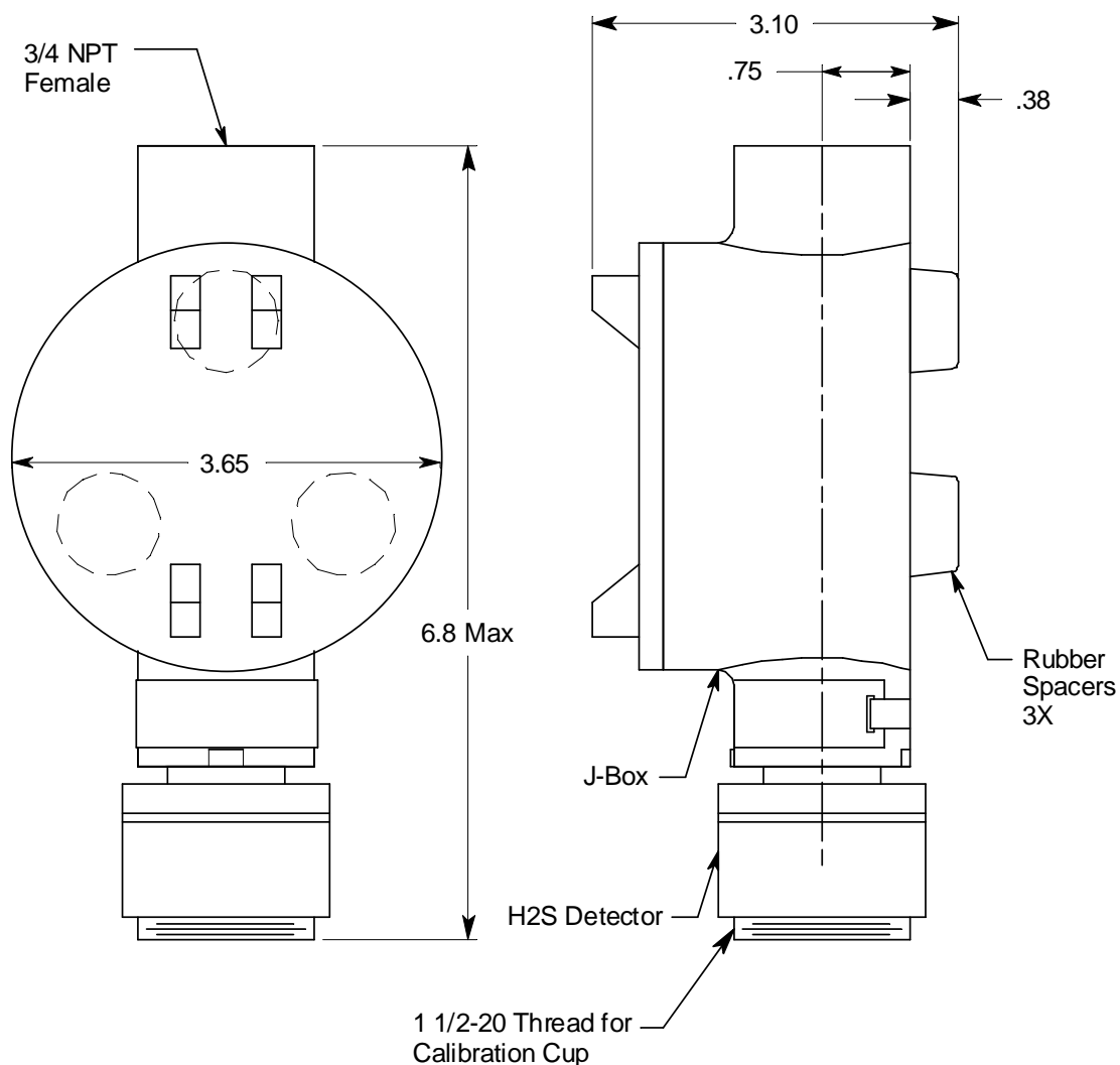
Figure 3: Mounting the H 2 S Transmitter
