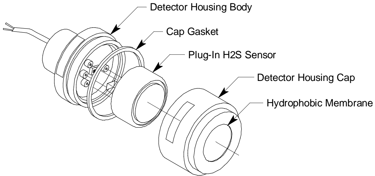
Figure 2: H 2 S Detector Component Location
