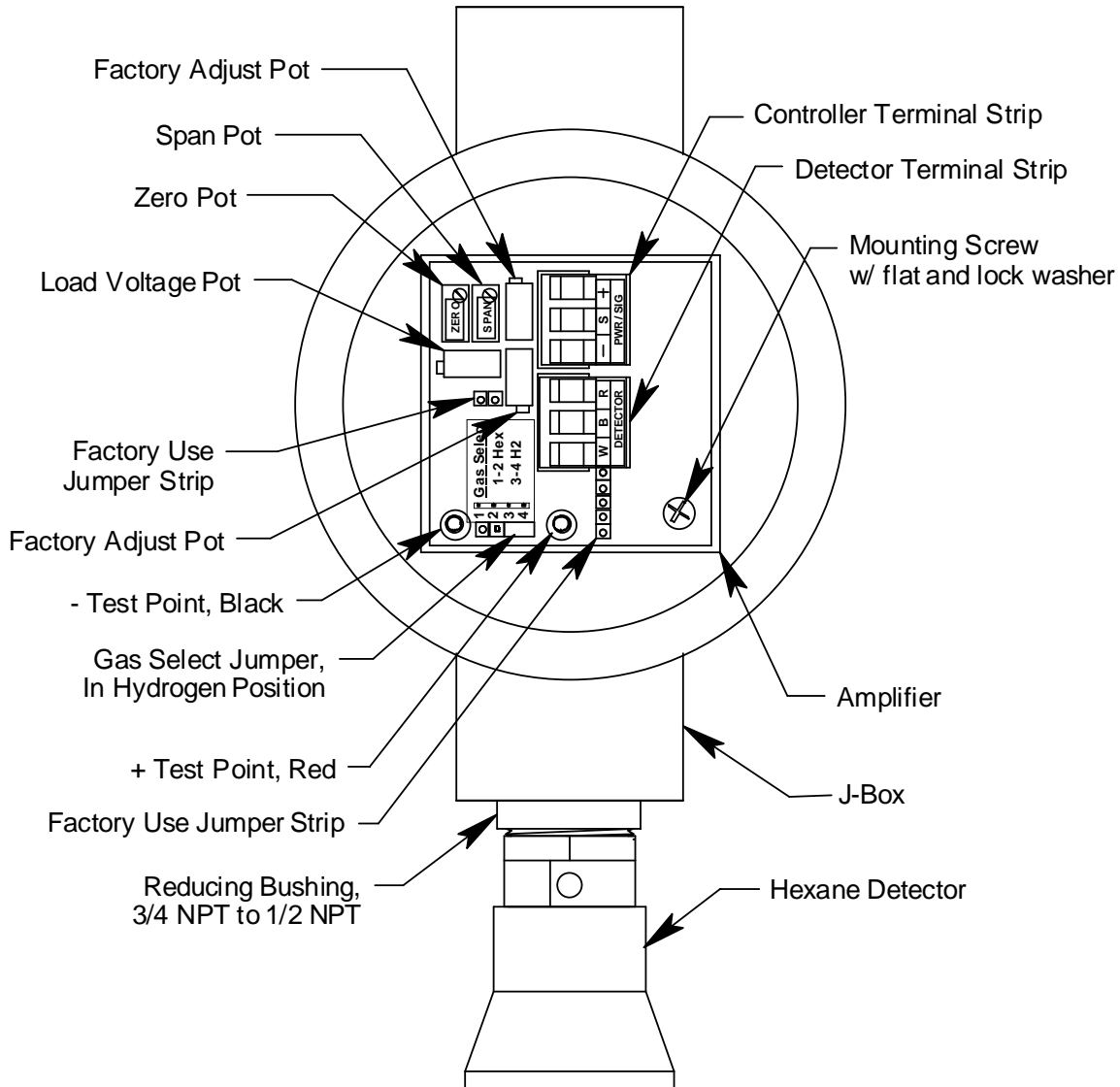
Figure 1: PPM Hexane Transmitter Component Location
