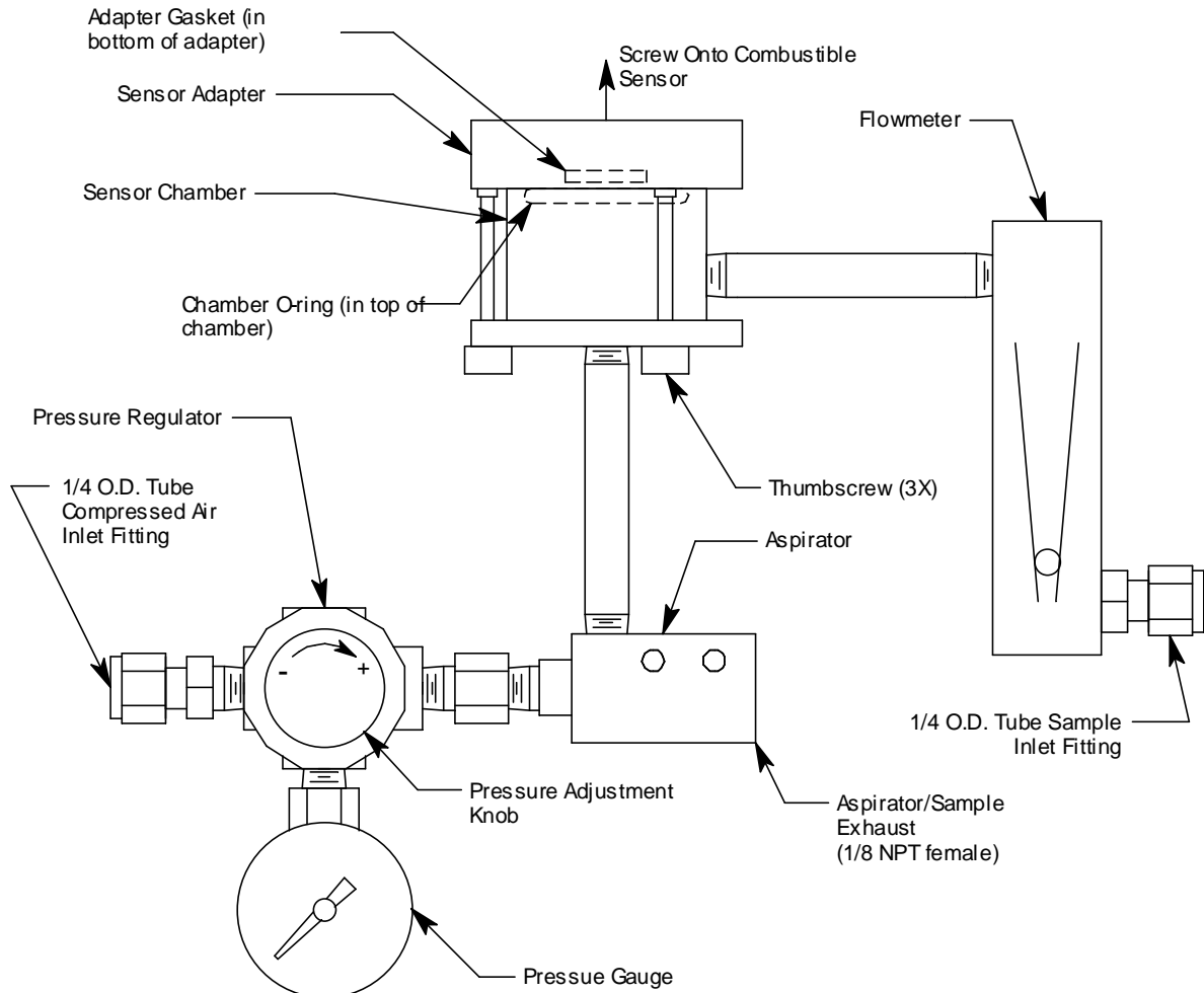
Figure 1: Component Location
