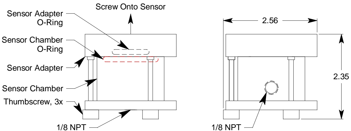
Figure 1: Outline and Mounting Dimensions/Component Location
