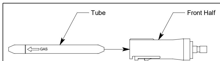
Figure 49: Inserting New Tube Into Front Half
