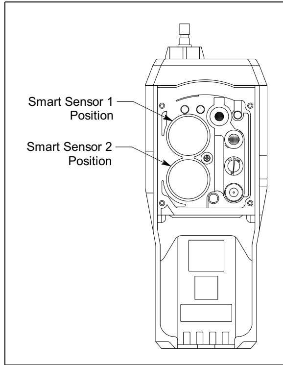
Figure 46: Smart Sensor Positions
