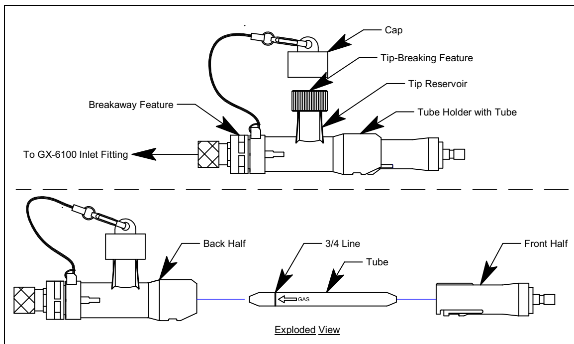
Figure 47: Tube Holder Component Location
