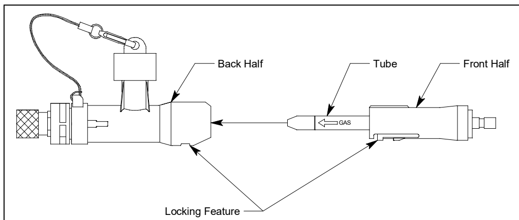
Figure 50: Reassembling Tube Holder
